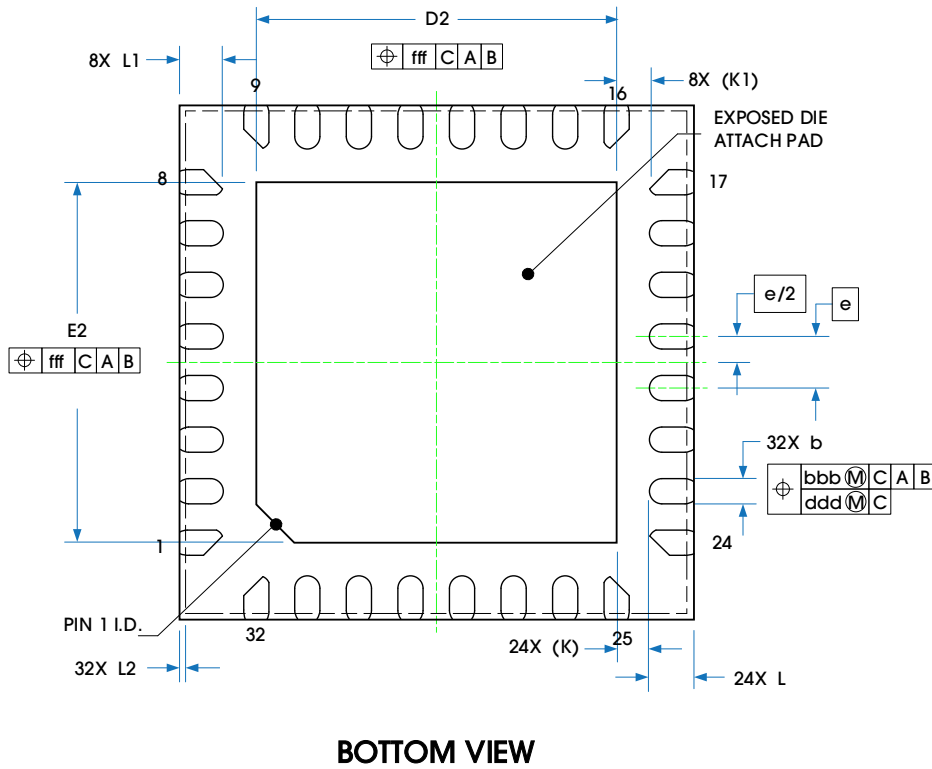
Figure 63. Package View
