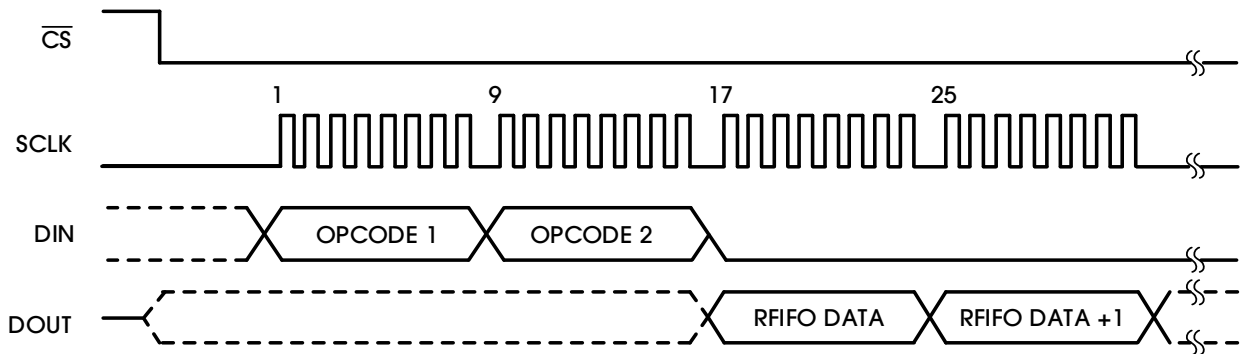
Figure 44. RFIFO Sequence
