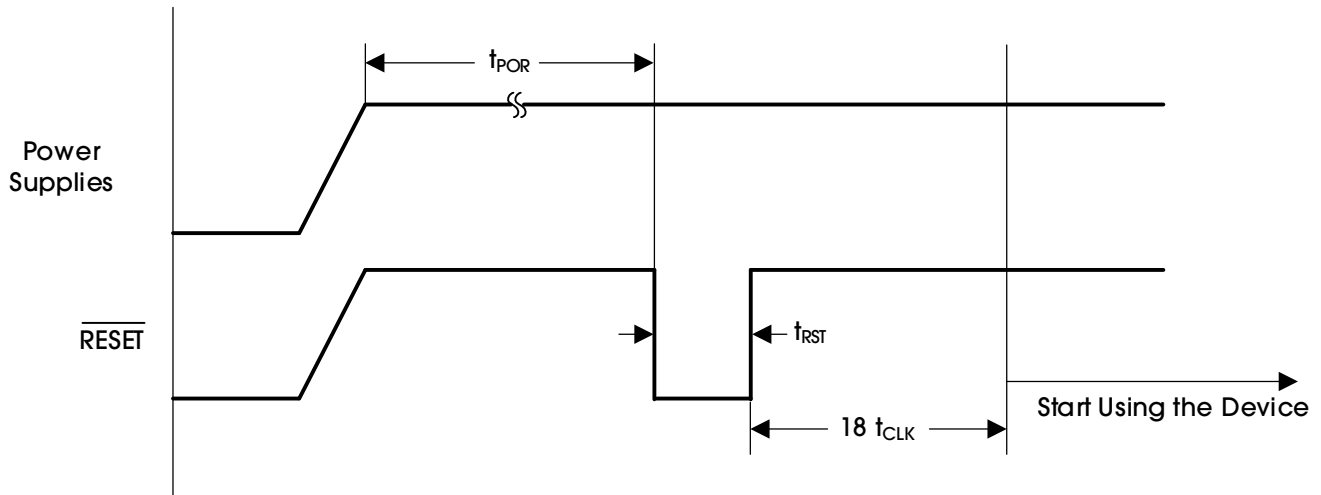
Figure 59. Power-Up Timing Diagram
