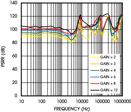
Figure 18. PSRR
