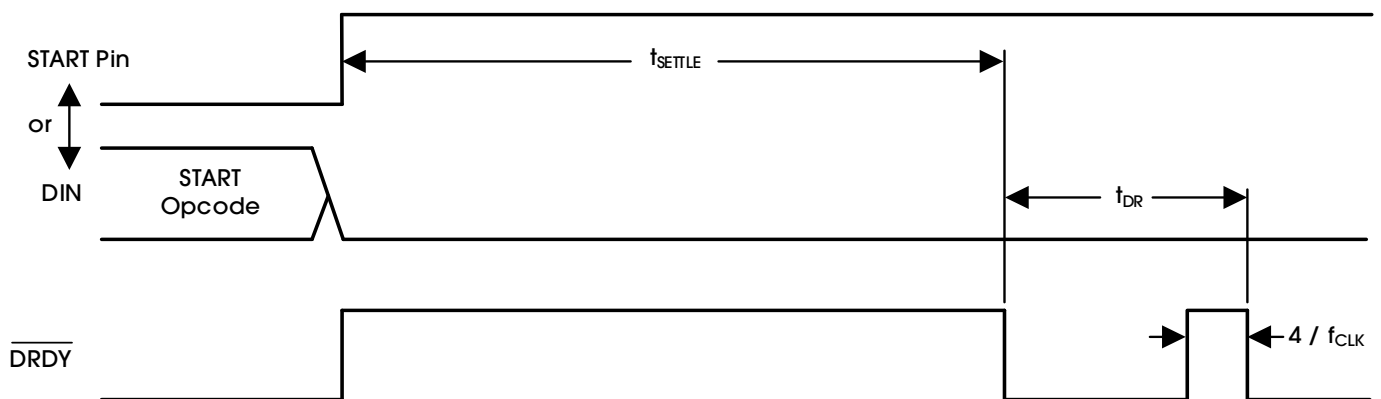
Figure 50. Settling Time
