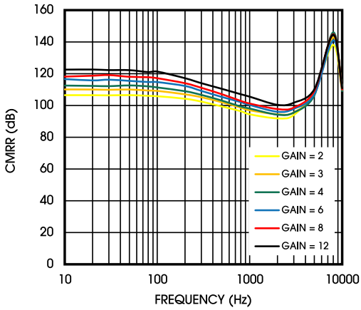
Figure 17. CMRR
