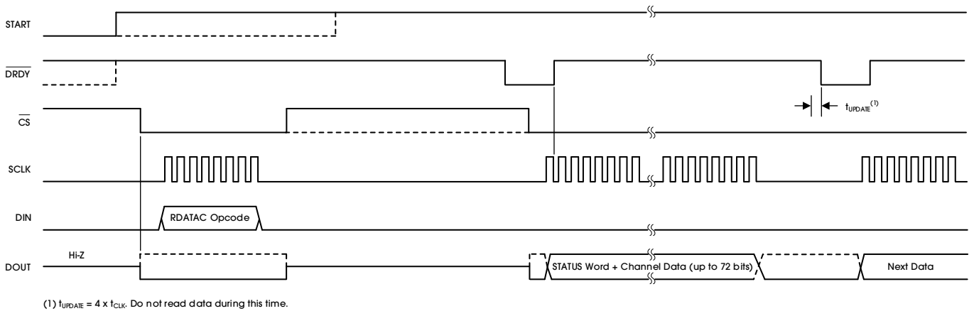
Figure 54. RDATA Usage
