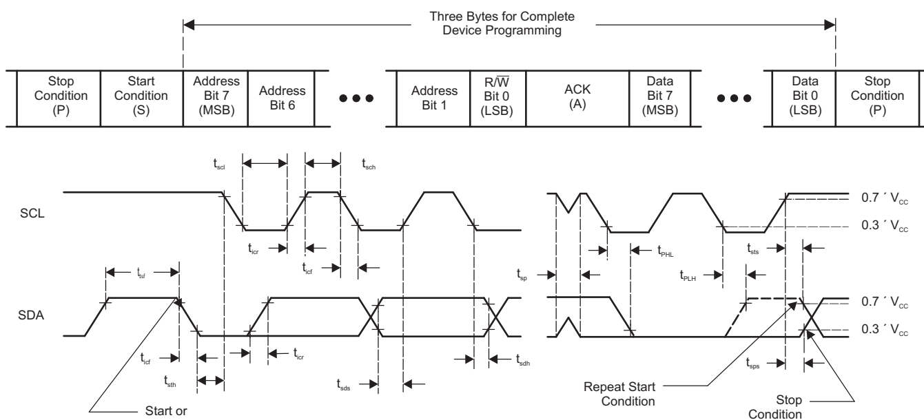
VOLTAGE WAVEFORMS
