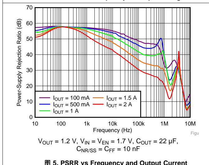
图 5. PSRR vs Frequency and Output Current
