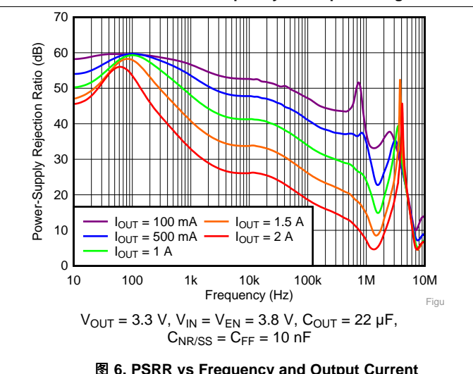
图 6. PSRR vs Frequency and Output Current
