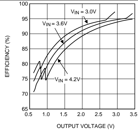
Figure 14. Efficiency vs Output Voltage
