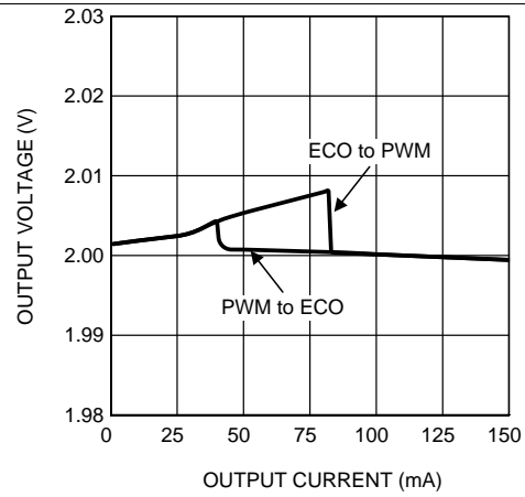
Figure 8. Output Voltage vs Output Current
