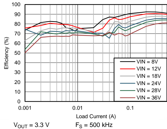
Figure 48. Efficiency
