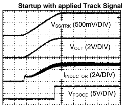
TIME (10 ms/DIV) Figure 24.
