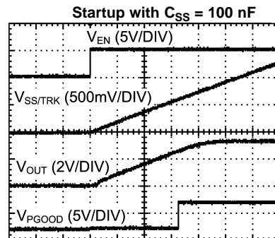
TIME (4 ms/DIV) Figure 23.
