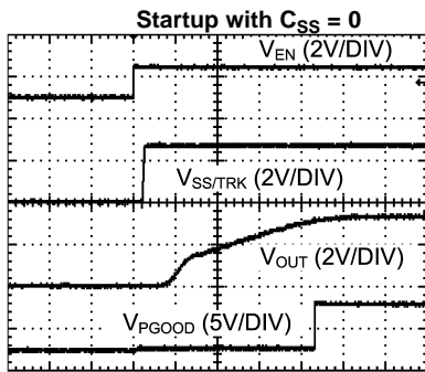
TIME (200 \mu s /DIV) Figure 22.
