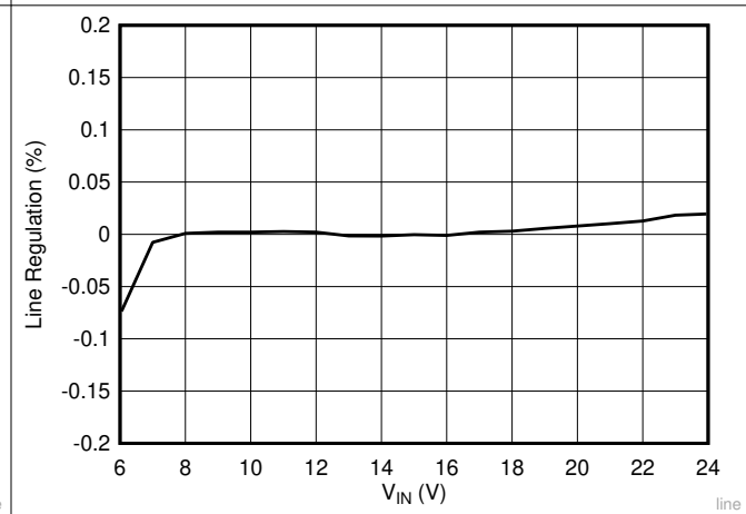
图 8-7. Line Regulation, I_{OUT} = 5\text{ A}
