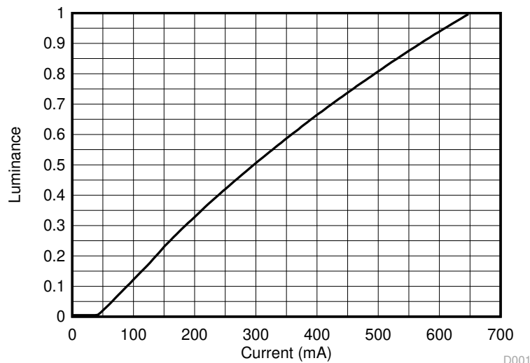
图 8-2. Typical Luminance vs Current
