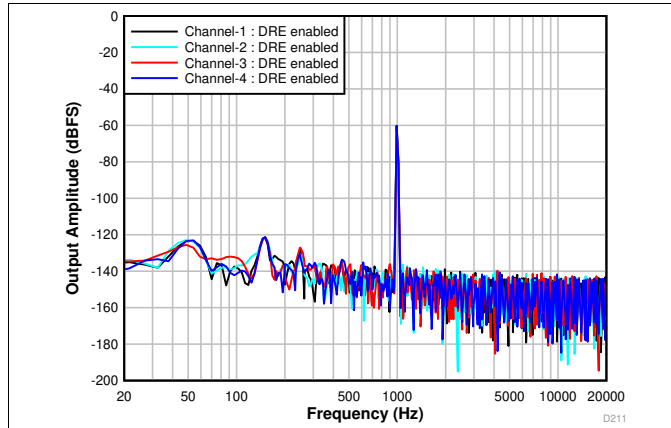
图 173. FFT With a -60-dBr Input With DRE Enabled
