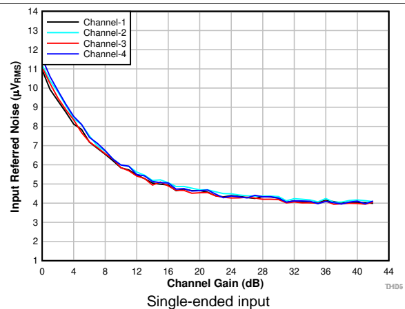
图 14. Input-Referred Noise vs Channel Gain
