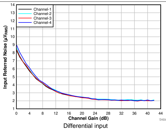
图 13. Input-Referred Noise vs Channel Gain
