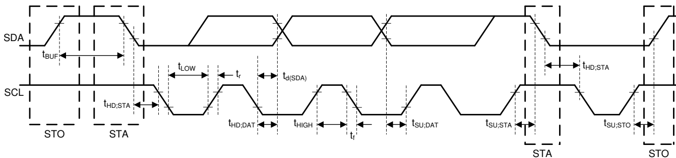
图 1. I 2 C Interface Timing Diagram
