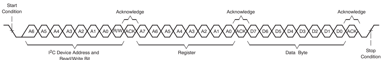
图 89. I 2 C Single-Byte Write Transfer
