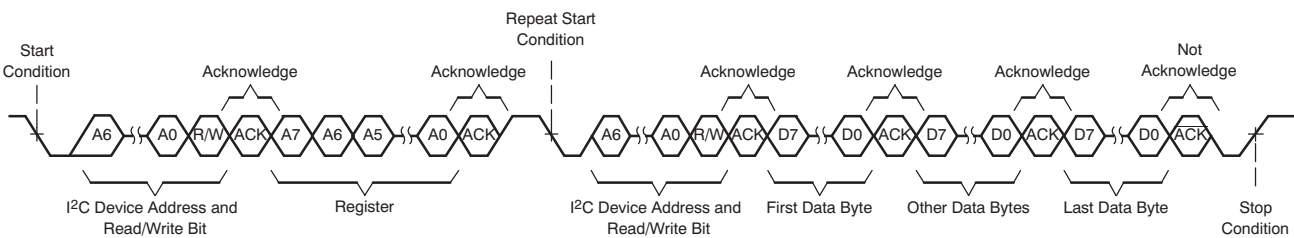
图 92. I 2 C Multiple-Byte Read Transfer
