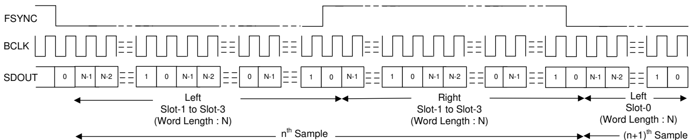
图 23. I 2 S Protocol Timing (No Idle BCLK Cycles, TX_OFFSET = 0)
