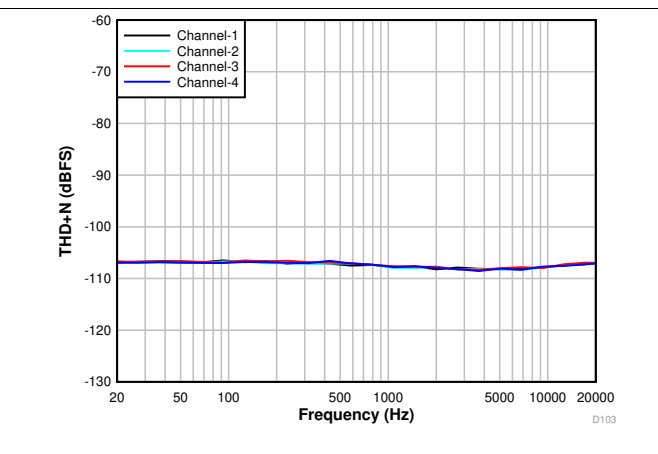
图 8. THD+N vs Input Frequency With a -60-dBr Input
