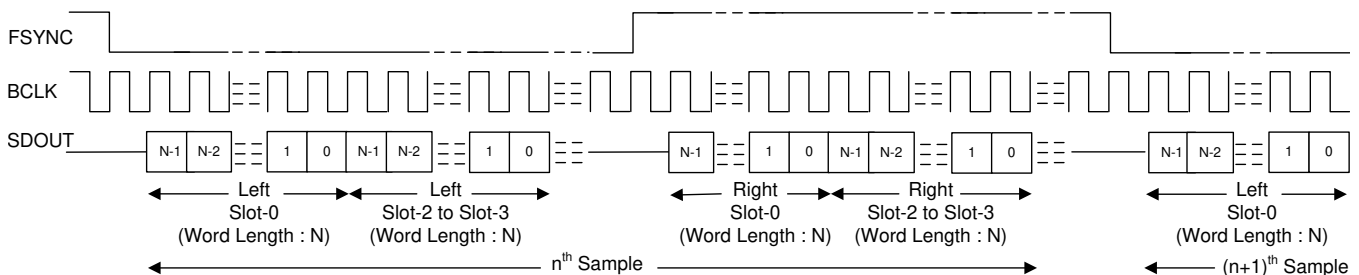
图 24. I 2 S Protocol Timing (TX_OFFSET = 0 and BCLK_POL = 1)
