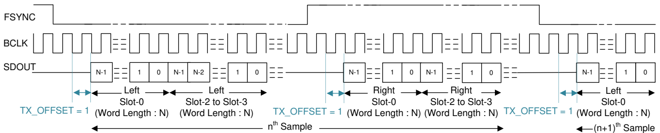
图 22. I 2 S Protocol Timing (TX_OFFSET = 1)
