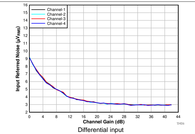
图 10. Input-Referred Noise vs Channel Gain
