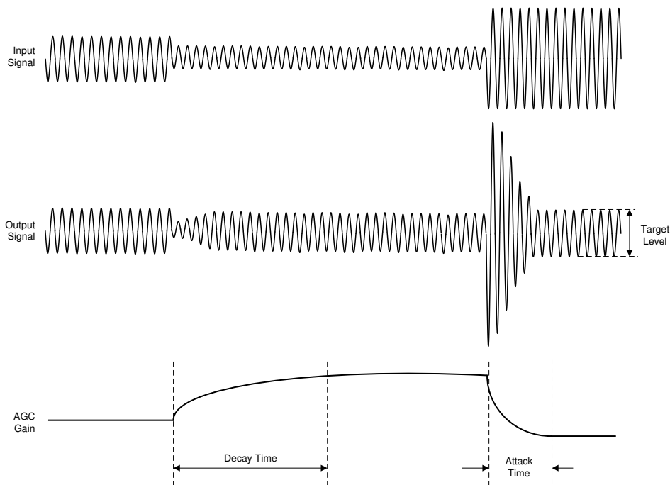
图 79. AGC Characteristics
