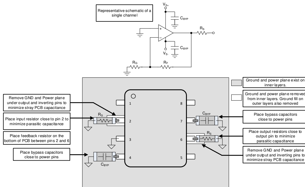
图 11-1. Layout Recommendation
