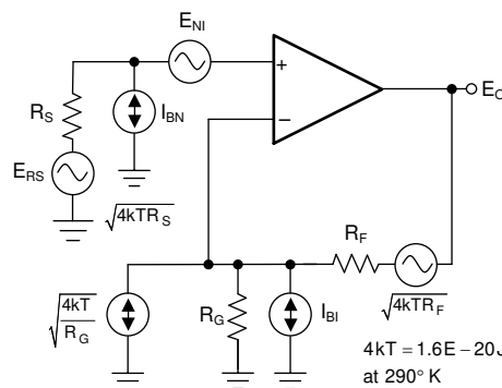
Figure 9-10. Operational Amplifier Noise Analysis Model
