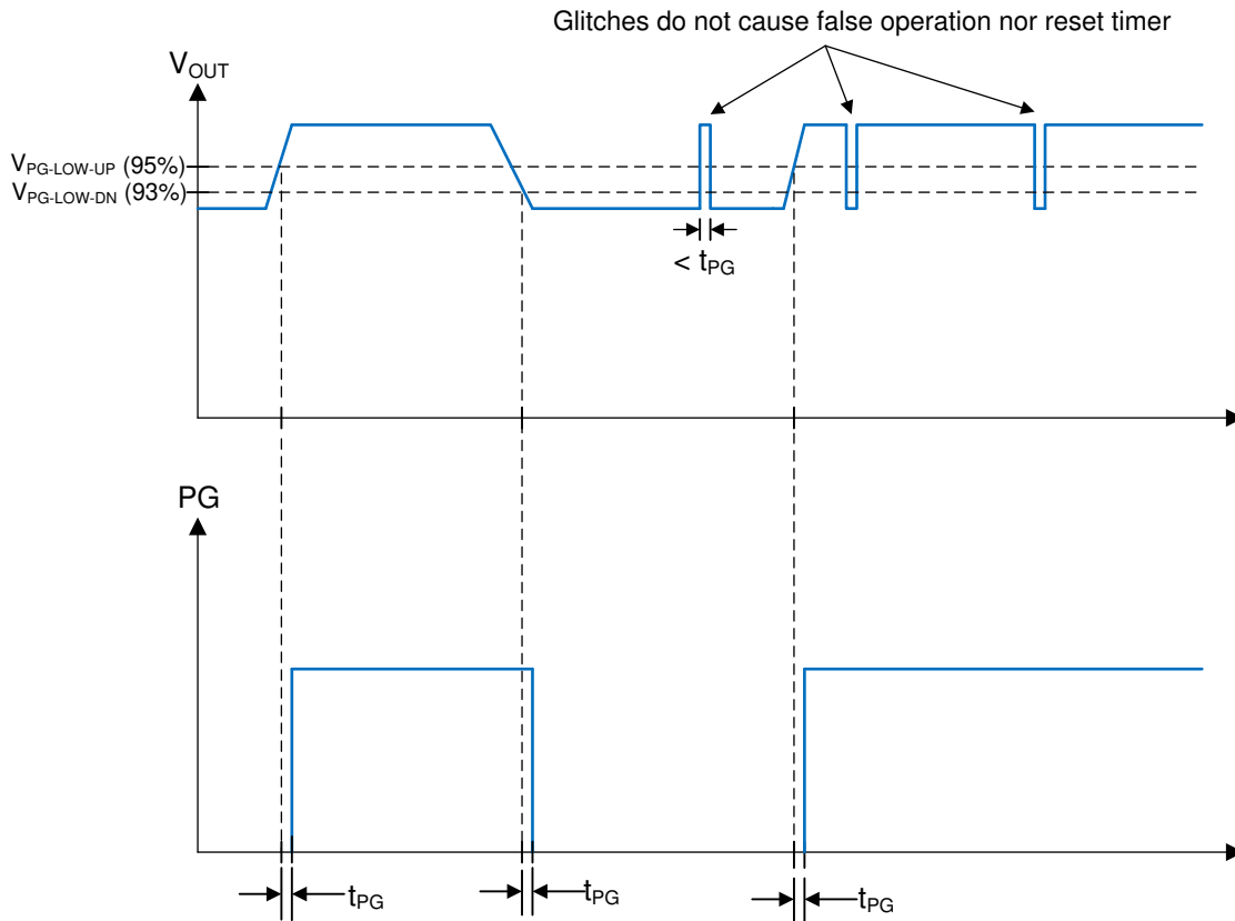
图 7-2. Power-Good-Timing Behavior
