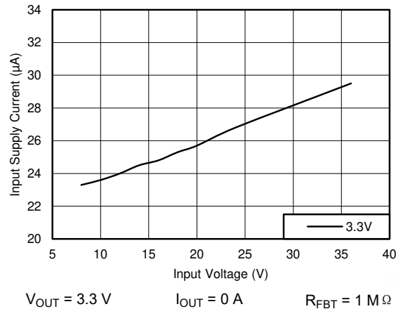
图 8-24. Input Supply Current
