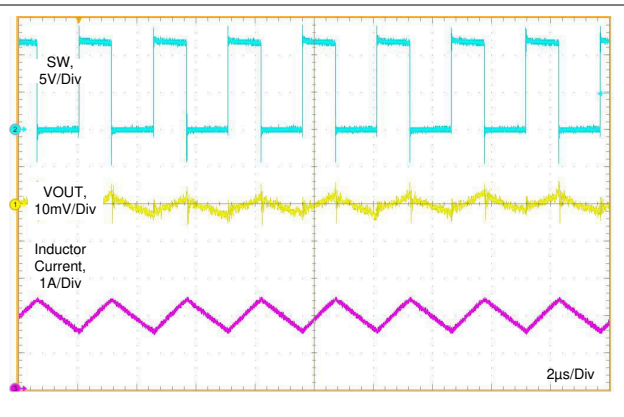
图 7-8. Typical PWM Switching Waveforms V_{IN} = 12 V, V_{OUT} = 5 V, I_{OUT} = 2 A, f_S = 400 kHz
