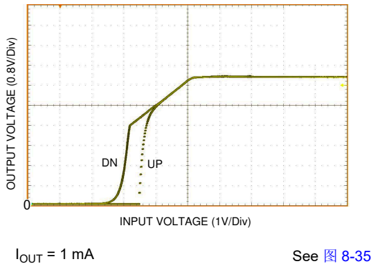
图 6-5. UVLO Thresholds
