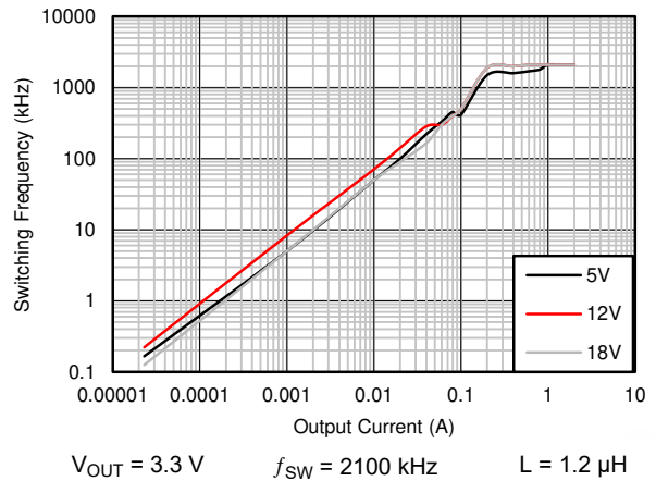
图 8-26. Switching Frequency versus Output Current
