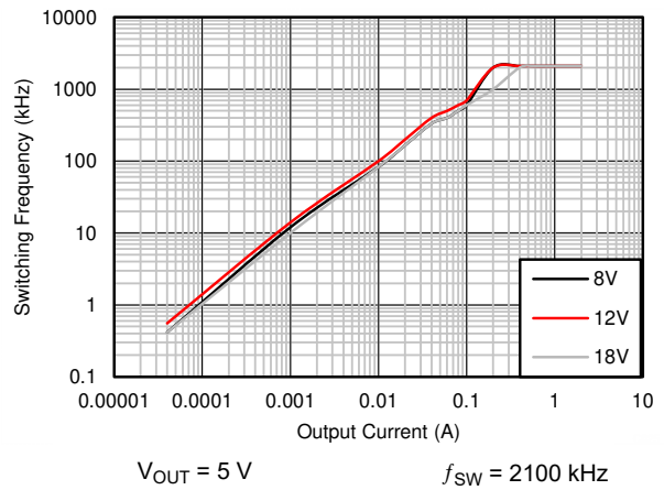
图 8-20. Switching Frequency versus Output Current
