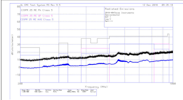
图 8-33. Radiated EMI Log-periodic Antenna (Vertical)
