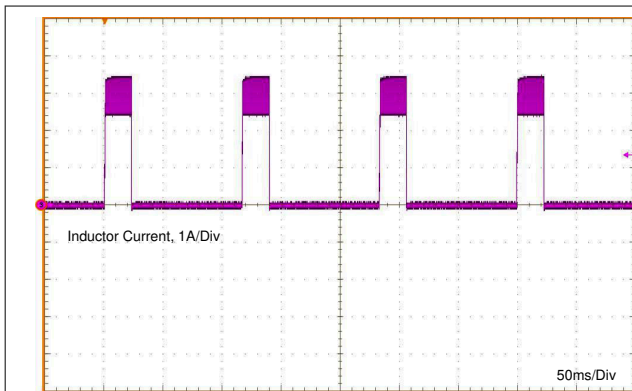
图 7-5. Inductor Current Burst in Short-Circuit Mode
