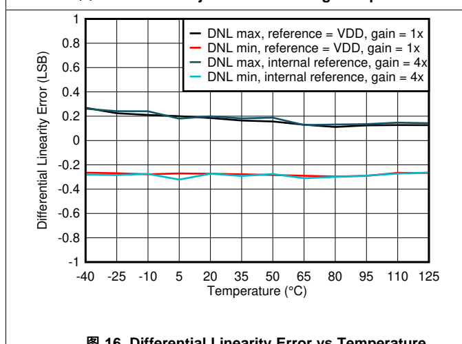
图 16. Differential Linearity Error vs Temperature
