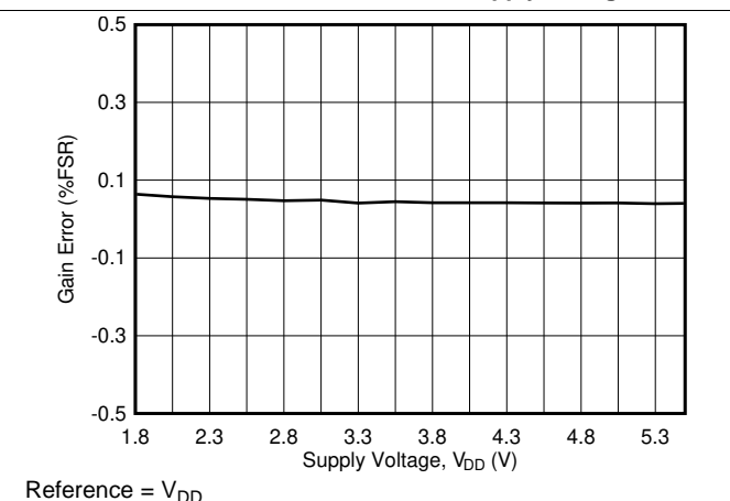
图 27. Gain Error vs Supply Voltage
