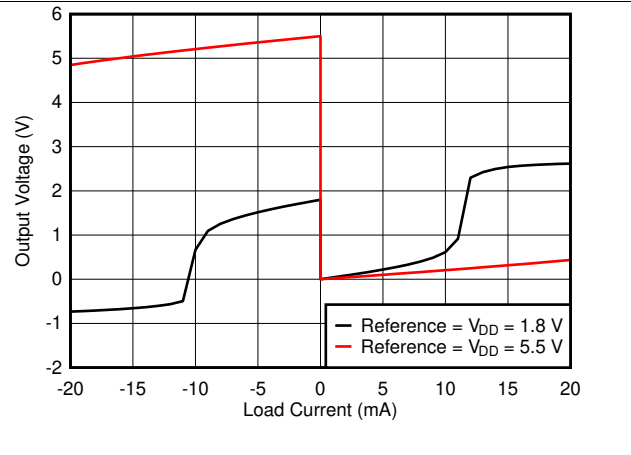
图 35. Source and Sink Capability
