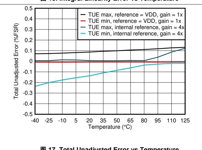
图 17. Total Unadjusted Error vs Temperature
