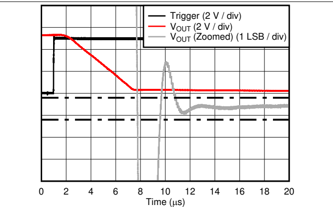
图 37. Glitch Impulse, Falling Edge, 1-LSB Step
