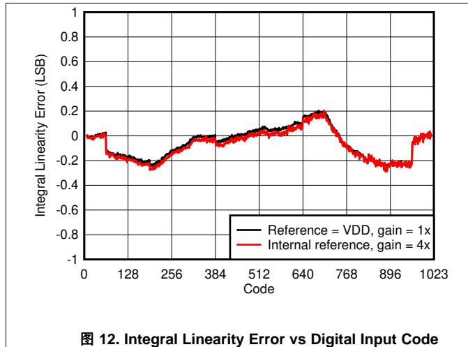
图 12. Integral Linearity Error vs Digital Input Code
