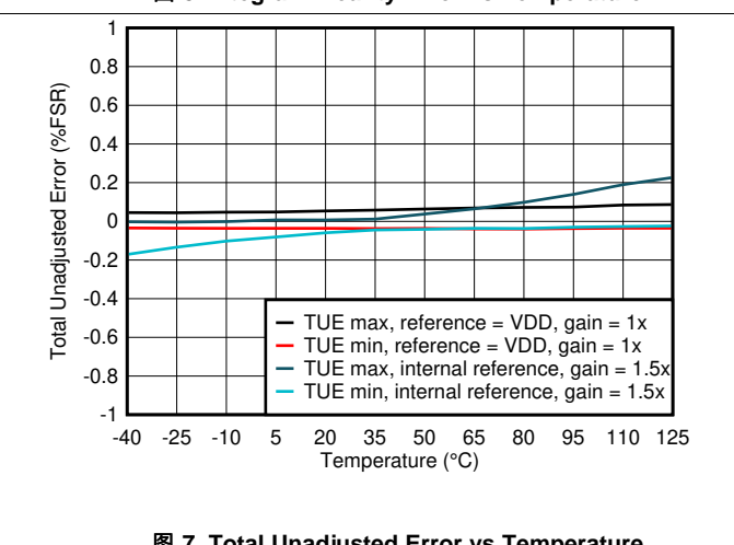
图 7. Total Unadjusted Error vs Temperature
