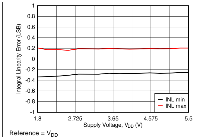
图 22. Integral Linearity Error vs Supply Voltage
