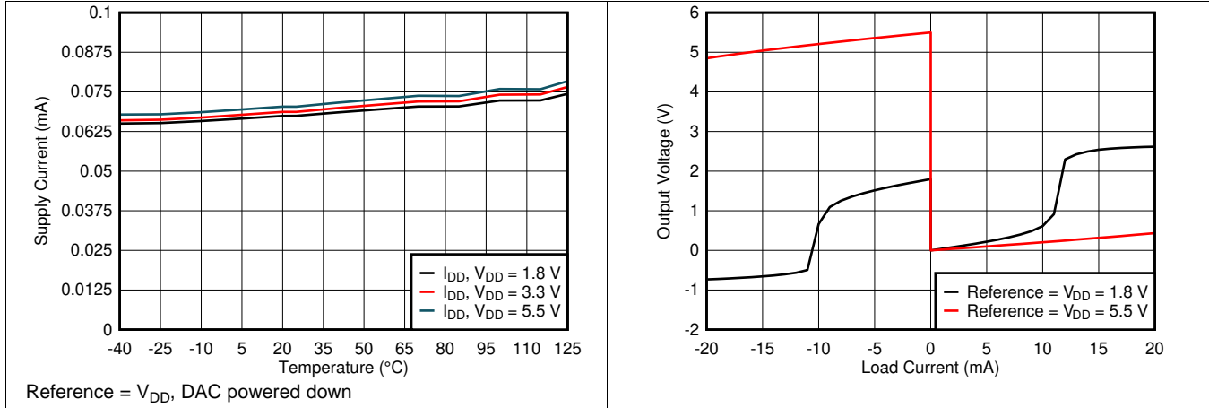
图 34. Power-Down Current vs Temperature
