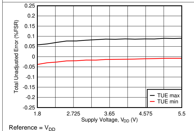
图 24. Total Unadjusted Error vs Supply Voltage
