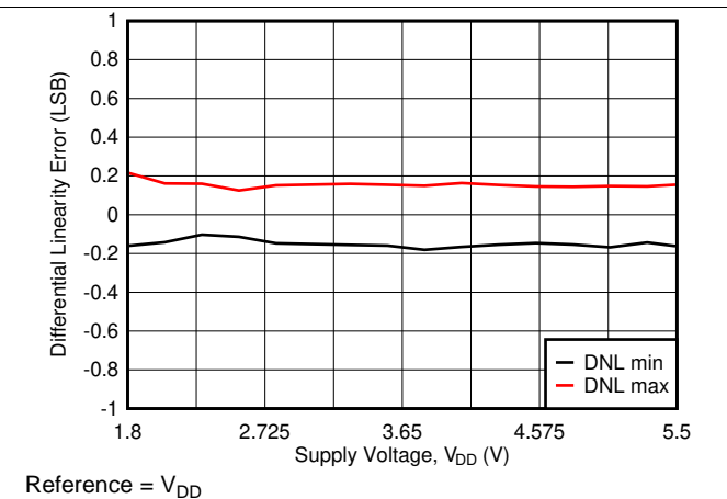
图 23. Differential Linearity Error vs Supply Voltage
