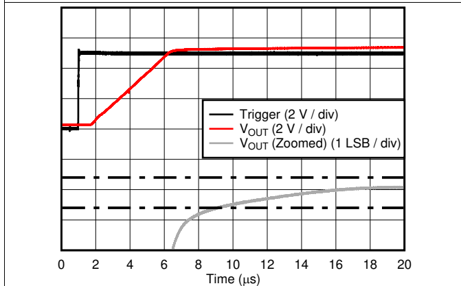
图 36. Glitch Impulse, Rising Edge, 1-LSB Step
