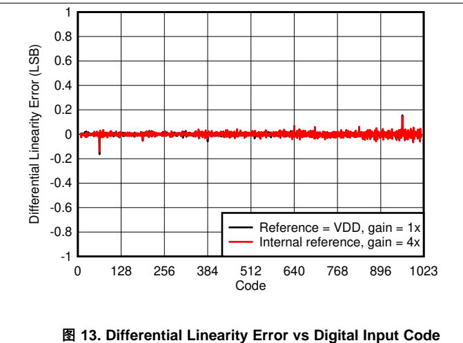
图 13. Differential Linearity Error vs Digital Input Code
