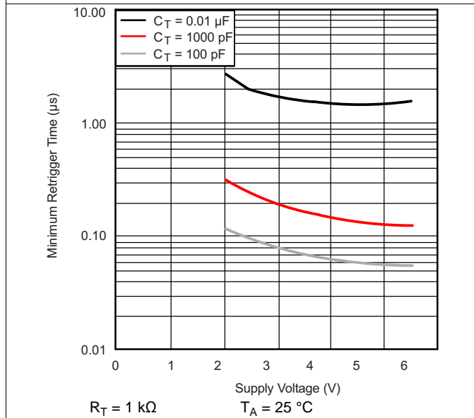
Figure 4. Minimum Trigger Time (t rr ) vs V CC Characteristics
