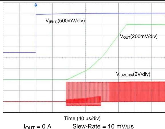
图 67. Start-Up With EN1, Forced PWM (2-Phase Output)
