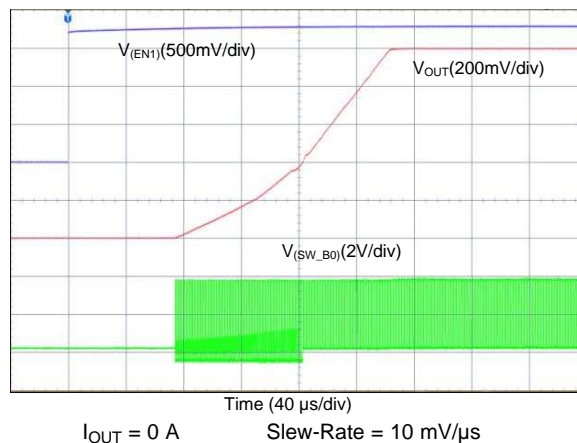
图 65. Start-Up With EN1, Forced PWM (4-Phase Output)
