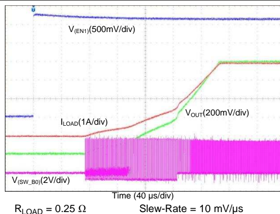
图 69. Start-Up With EN1, Forced PWM (4-Phase Output)
