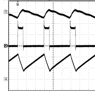
V_{IN} = 3.6V , 4 LEDs, I_{LED} = 30mA , V_{OUT} = 15.8V Channel 1: V_{OUT} (AC Coupled, 100mV/div) Channel 2: V_{SW} (DC Coupled, 10V/div) Channel 4: I_L (DC Coupled, 100mA/div) Time Base: 400ns/div
