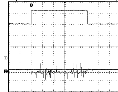
CH1: V_{IN} ; Scale: 1V/Div, DC Coupled CH2: V_{OUT} ; Scale: 20mV/Div, AC Coupled Time scale: 10ms/Div
