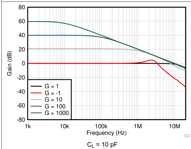
图 7-55. Closed-Loop Gain vs Frequency
