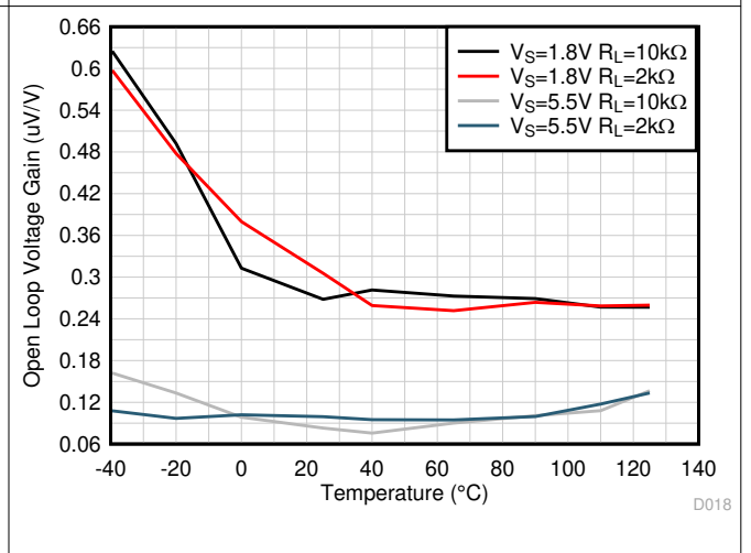
图 7-56. Open-Loop Gain vs Temperature
