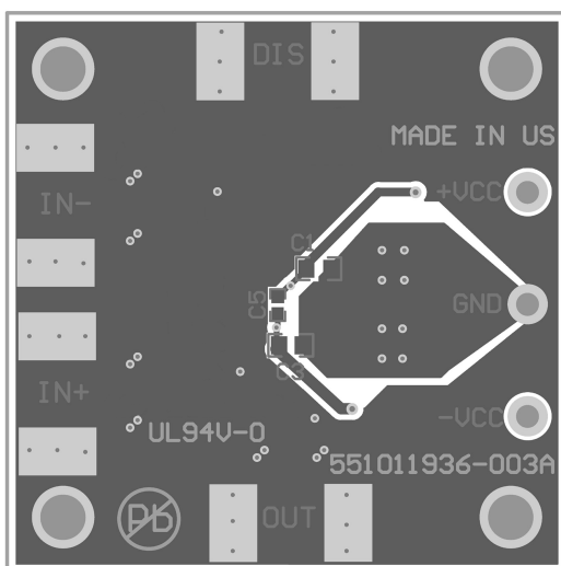
Figure 48. Layer 2 Silks (SOT-23 Board Layout)
