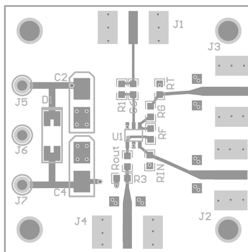
Figure 49. Layer 1 Silks (SOT-23 Board Layout)
