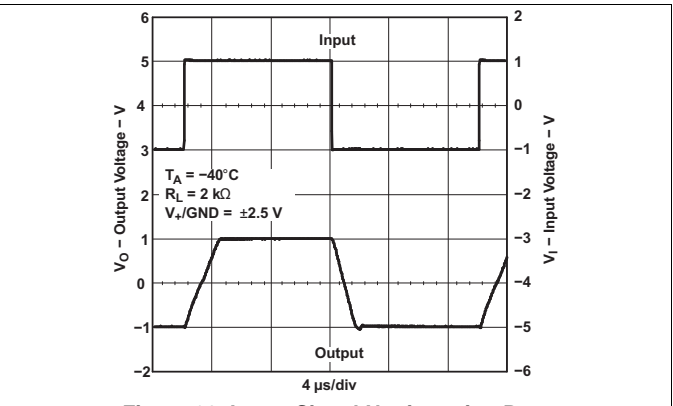
Figure 26. Large-Signal Noninverting Response
