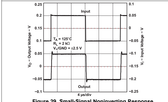
Figure 29. Small-Signal Noninverting Response
