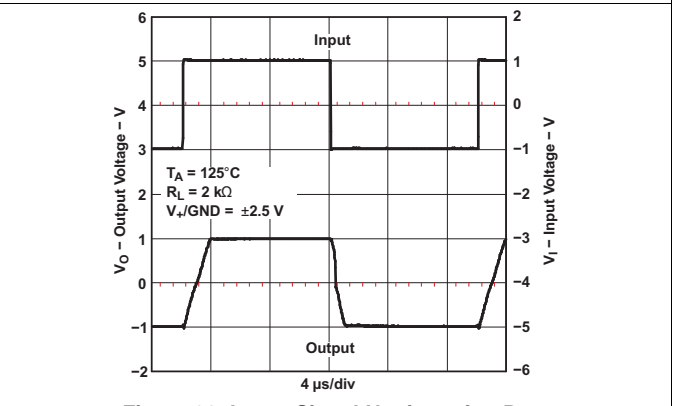
Figure 30. Large-Signal Noninverting Response
