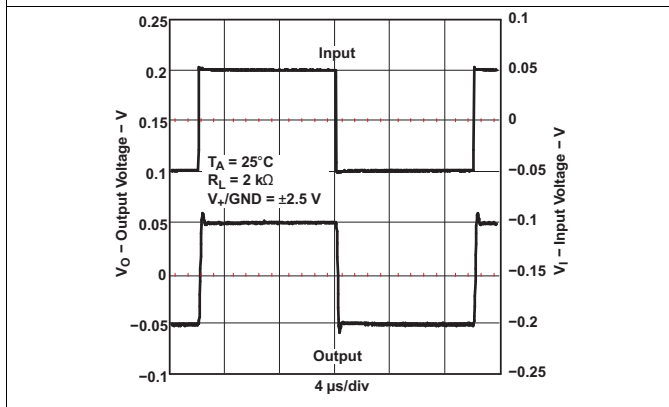
Figure 27. Small-Signal Noninverting Response
