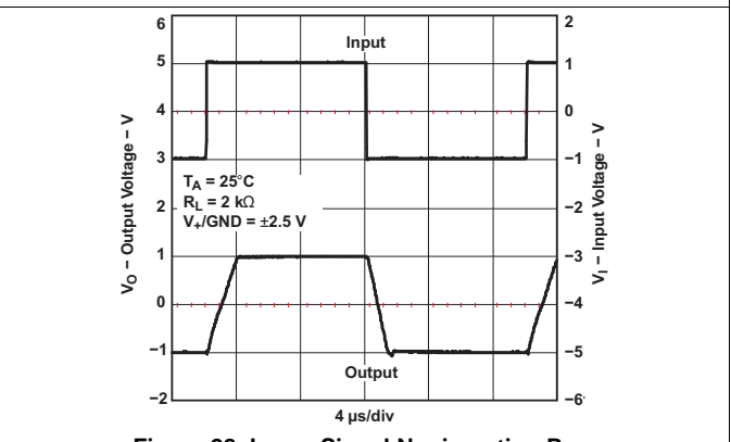
Figure 28. Large-Signal Noninverting Response
