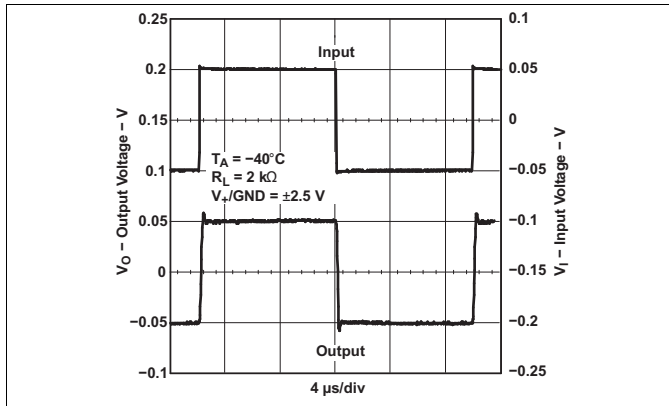
Figure 25. Small-Signal Noninverting Response
