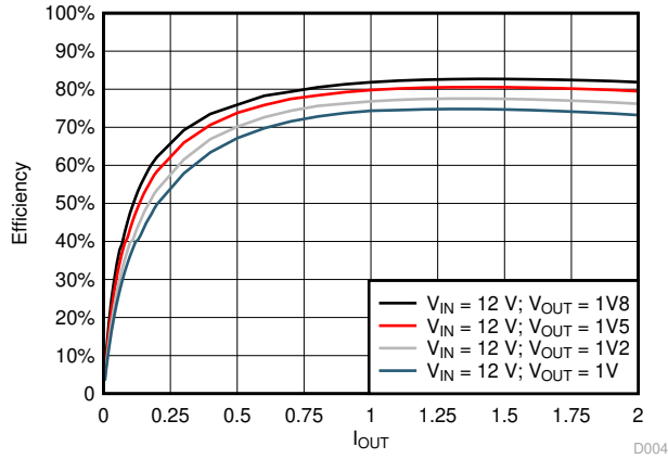
图 7-3. Buck3 and Buck4 Power Efficiency, V_{IN} = 12\text{ V}
