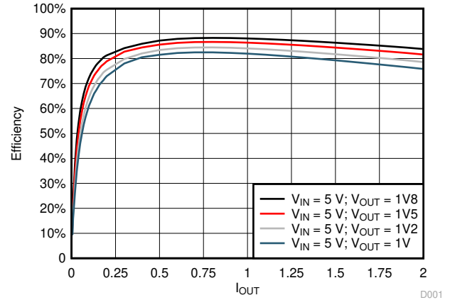
图 7-4. Buck3 and Buck4 Power Efficiency, V_{IN} = 5\text{ V}
