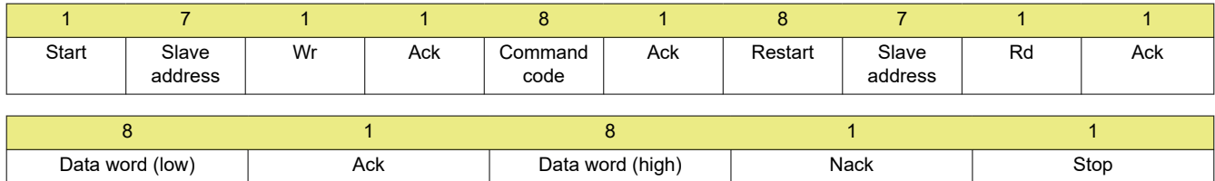
图 8-25. Read Word Protocol
