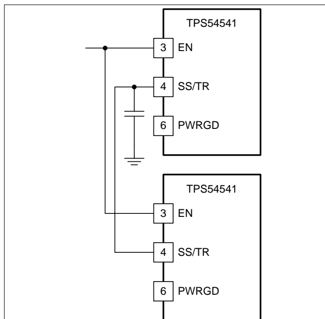
Figure 31. Schematic for Ratiometric Startup Sequence
