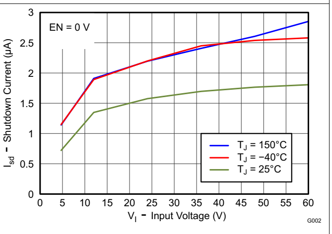
Figure 12. Shutdown Supply Current (VIN) vs Input Voltage
