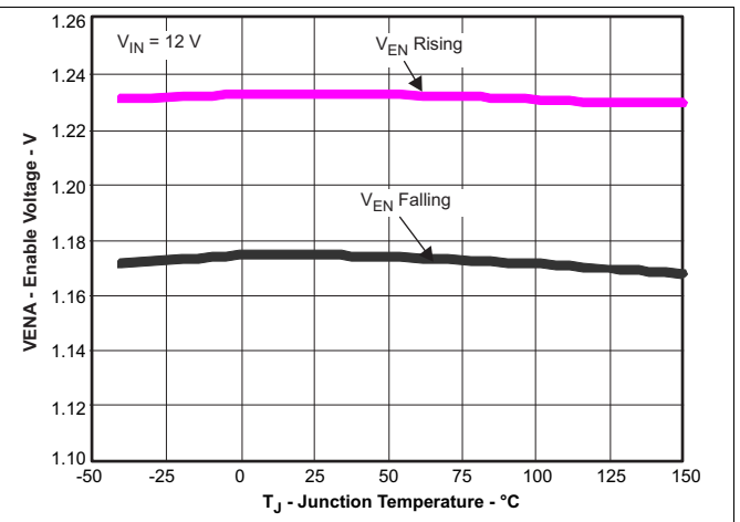
Figure 8. Enable Pin Voltage vs Temperature
