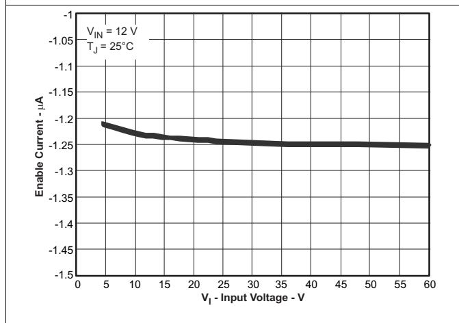
Figure 11. Enable Pin Pullup Current vs Input Voltage
