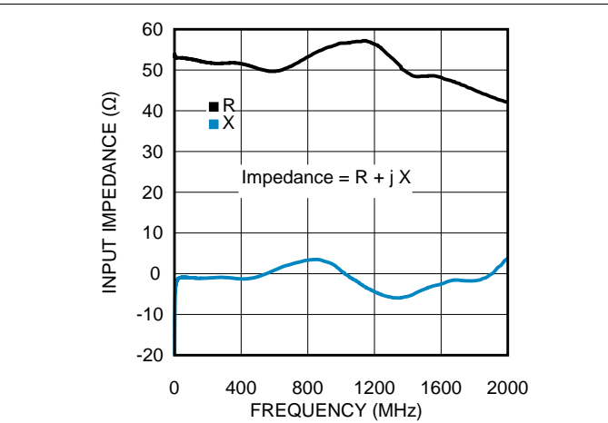
Figure 38. Input Impedance
