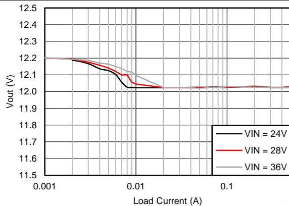
Figure 9. V_{OUT} Regulation
