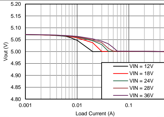
Figure 7. V_{OUT} Regulation
