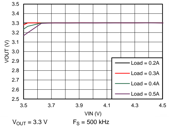
Figure 56. Dropout Curve
