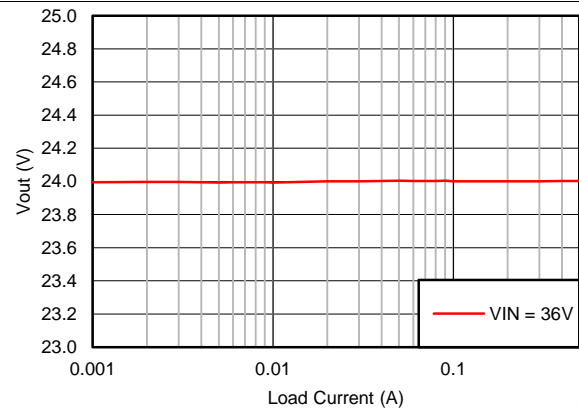
Figure 10. V_{OUT} Regulation
