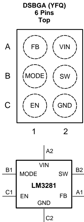
Figure 1. Pin Out
