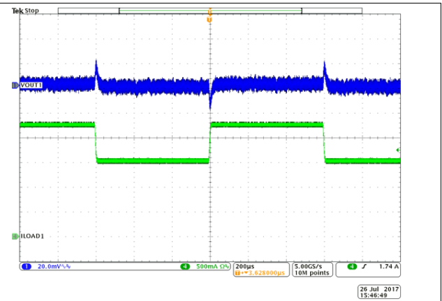
I_{OUT} = 1.5 to 2.25 A SR = 0.25 A/ \mu s
