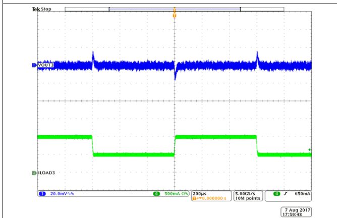
I_{OUT} = 0.5 to 1 A SR = 0.25 A/ \mu s
