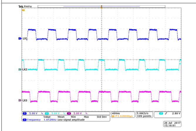
图 50. 180° Out-of-Phase
