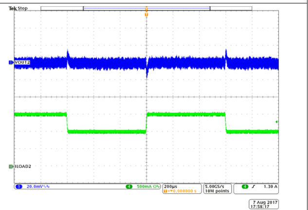
I_{OUT} = 1 to 1.5 A SR = 0.25 A/ \mu s
