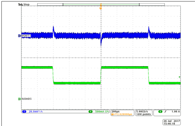
I_{OUT} = 0.75 to 1.5 A SR = 0.25 A/ \mu s
