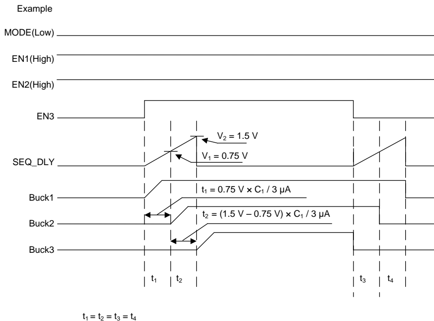
Figure 28. Automatic Power Sequencing
