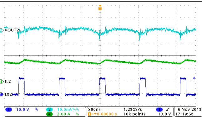
Figure 51. Buck2, PSM Mode, Output Ripple, Light Load
