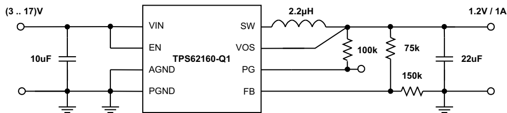
Figure 36. 1.2-V/1-A Power Supply
