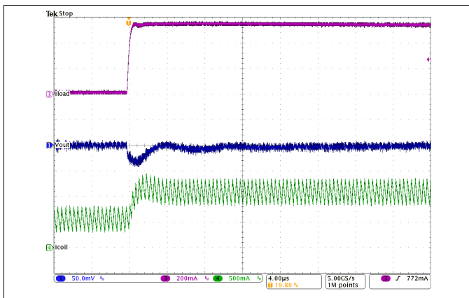
Figure 24. Load Transient Response in PWM Mode
