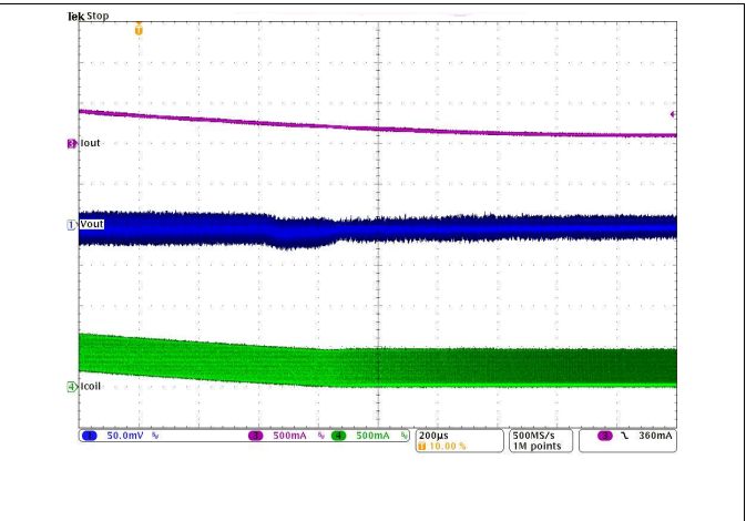
Figure 21. PWM to PSM Mode Transition
