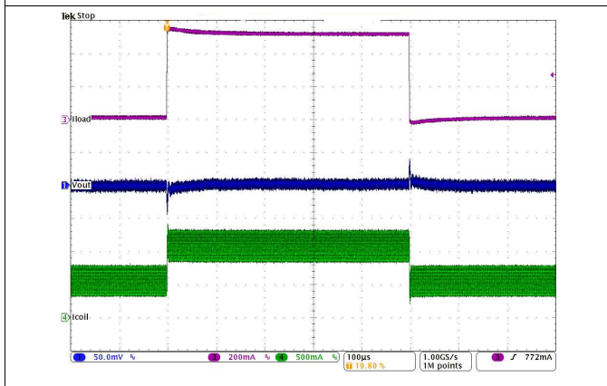
Figure 20. PWM / PSM Mode Transitions
