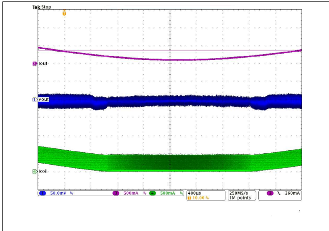
Figure 20. PWM / PSM Mode Transitions
