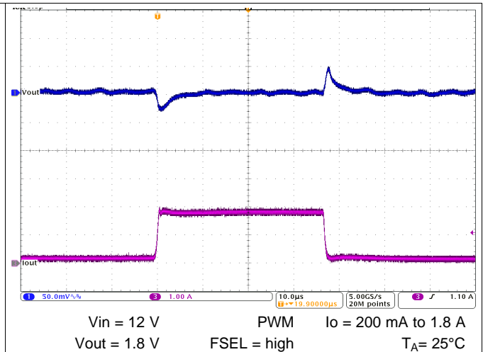
图 43. Load Transient Response
