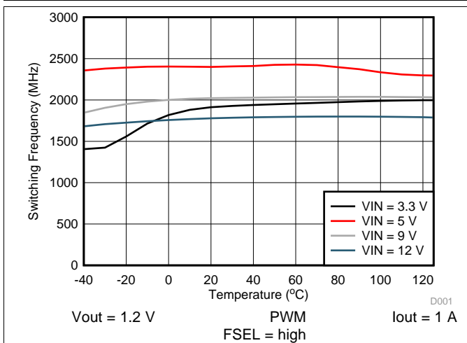
图 72. Switching Frequency vs Junction Temperature
