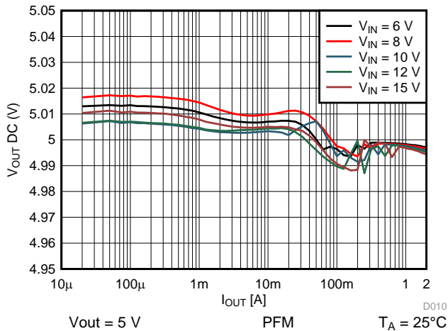
图 32. Output Voltage vs Output Current
