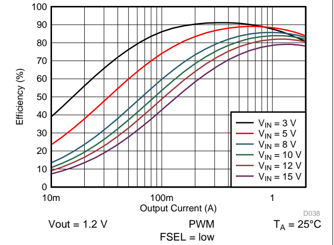
图 9. Efficiency vs Output Current
