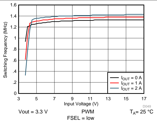
图 77. Switching Frequency vs Input Voltage
