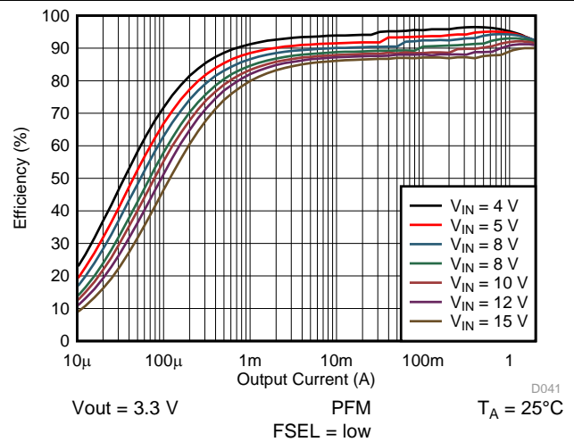
图 15. Efficiency vs Output Current
