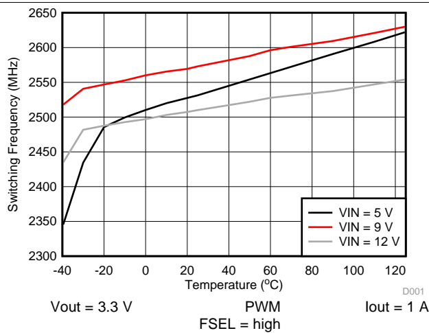
图 78. Switching Frequency vs Junction Temperature
