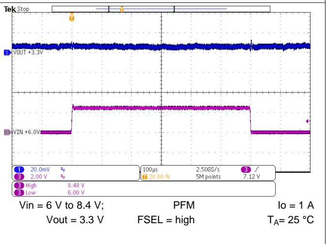
图 51. Line Transient Response
