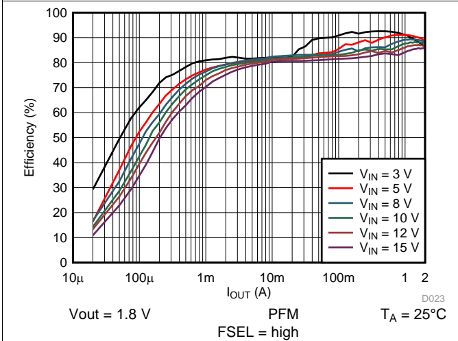
图 10. Efficiency vs Output Current
