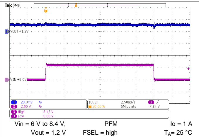
图 37. Line Transient Response
