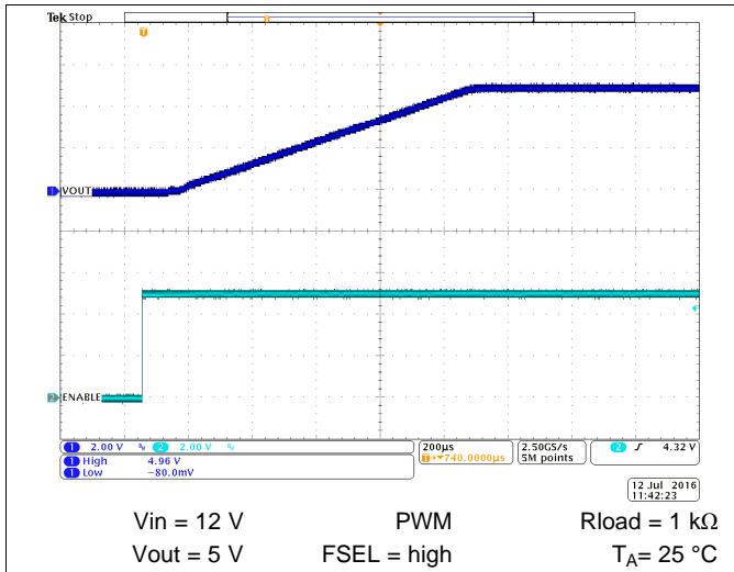
图 60. Start-Up Timing
