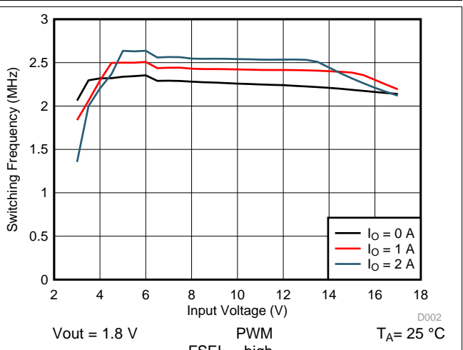
图 73. Switching Frequency vs Input Voltage
