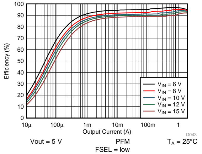
图 19. Efficiency vs Output Current
