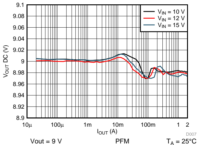
图 34. Output Voltage vs Output Current
