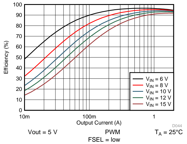
图 21. Efficiency vs Output Current
