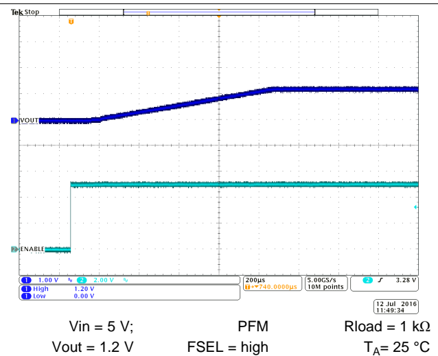
图 39. Start-Up Timing
