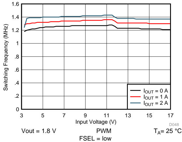
图 74. Switching Frequency vs Input Voltage
