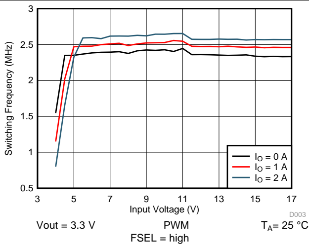
图 76. Switching Frequency vs Input Voltage
