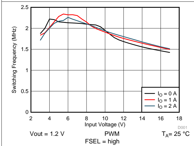
图 70. Switching Frequency vs Input Voltage
