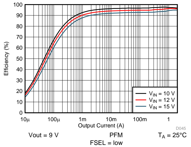
图 23. Efficiency vs Output Current
