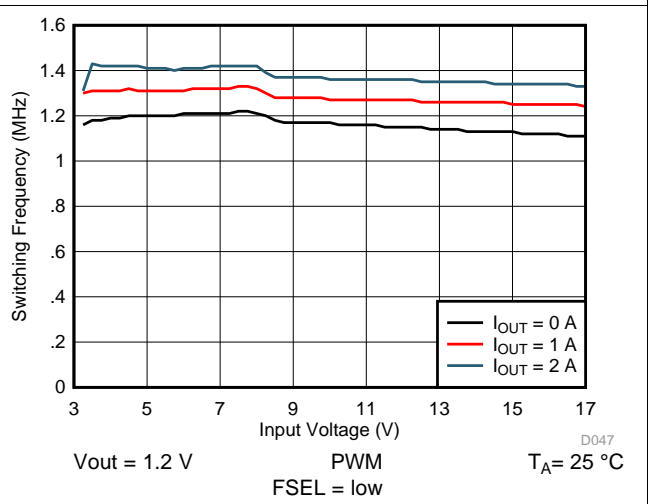
图 71. Switching Frequency vs Input Voltage
