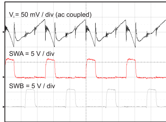
图 55. Full Load Input Voltage Ripple
