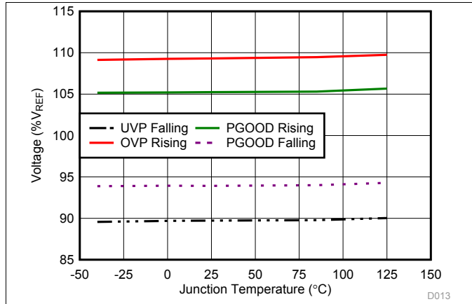
图 13. PGOOD and Under/Overvoltage Protection Threshold vs Junction Temperature
