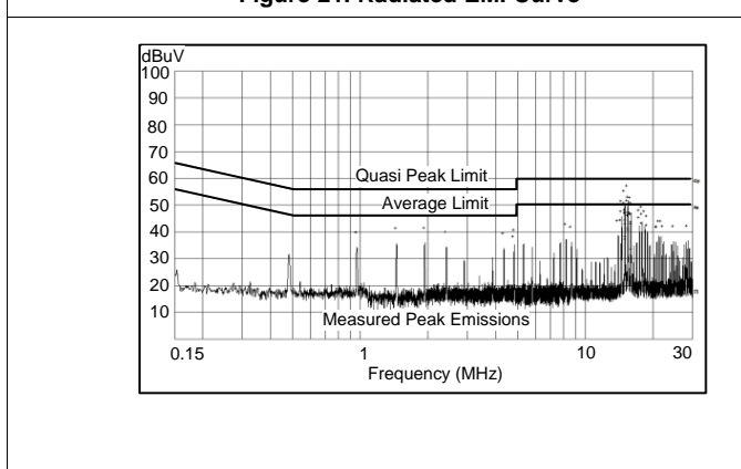
Figure 21. Radiated EMI Curve
