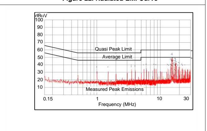
Figure 22. Radiated EMI Curve
