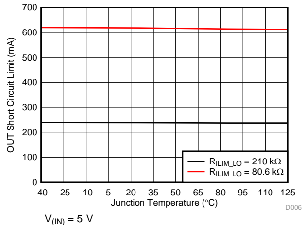
Figure 6. OUT Short-Circuit Current Limit vs Temperature II
