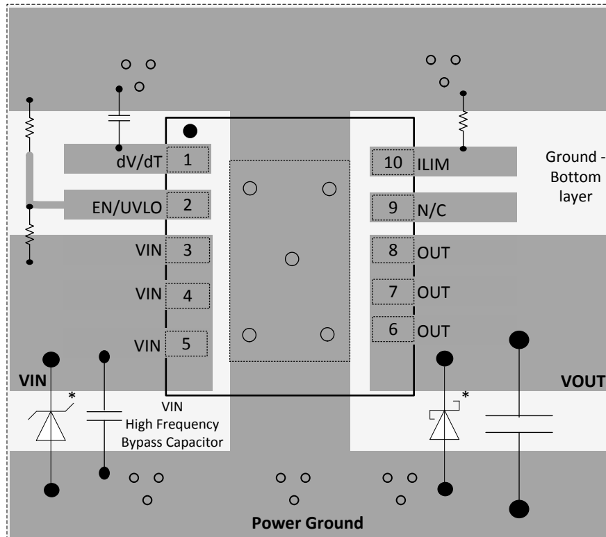
Figure 47. Layout Example
