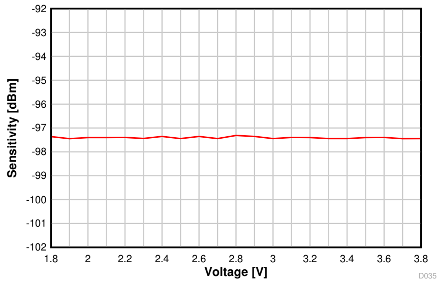
图 8-13. Sensitivity vs. Supply Voltage (VDD5) (BLE 1 Mbps, 2.44 GHz, DCDC Off)
