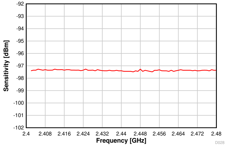
图 8-10. Sensitivity vs. Frequency (BLE 1 Mbps, 2.44 GHz)
