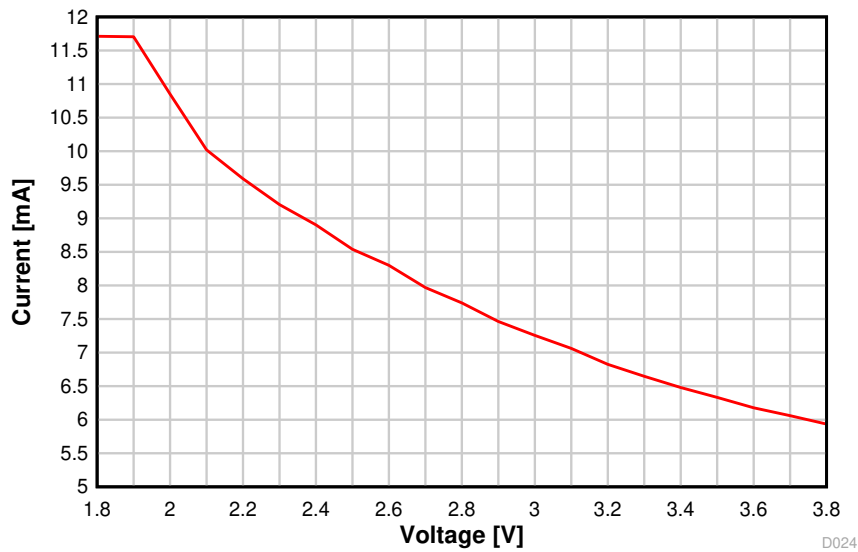
图 8-9. TX Current vs. Supply Voltage (VDD5) (BLE 1 Mbps, 2.44 GHz)
