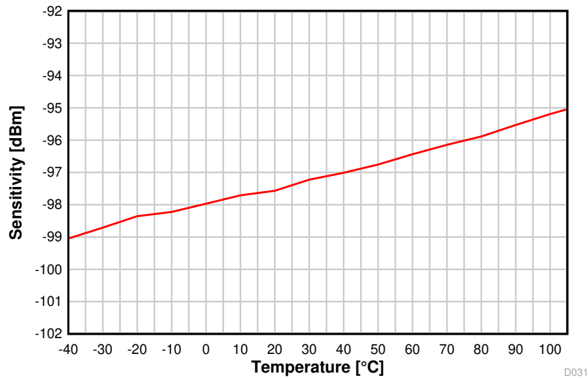
图 8-11. Sensitivity vs. Temperature (BLE 1 Mbps, 2.44 GHz)
