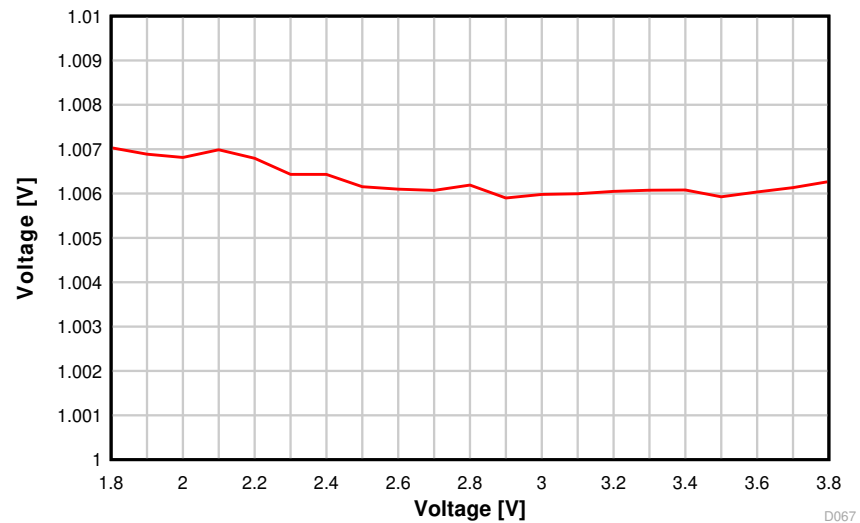
图 8-25. ADC Accuracy vs. Supply Voltage (VDDS)
