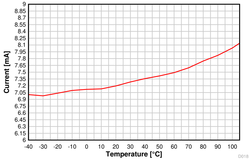
图 8-8. TX Current vs. Temperature (BLE 1 Mbps, 2.44 GHz)
