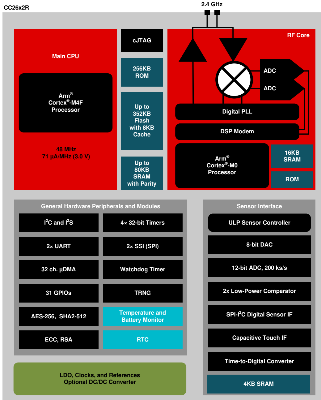
图 4-1. CC2642R Block Diagram
