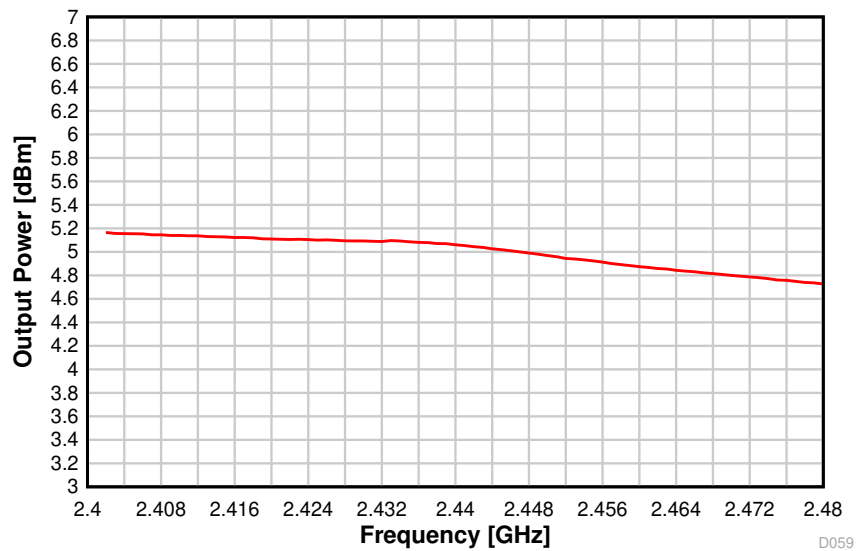
图 8-19. Output Power vs. Frequency (BLE 1 Mbps, 2.44 GHz, +5 dBm)
