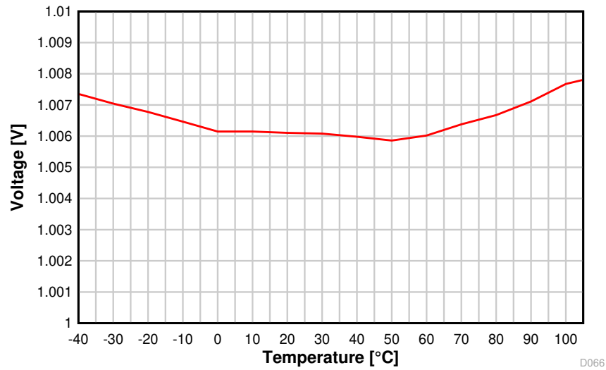
图 8-24. ADC Accuracy vs. Temperature
