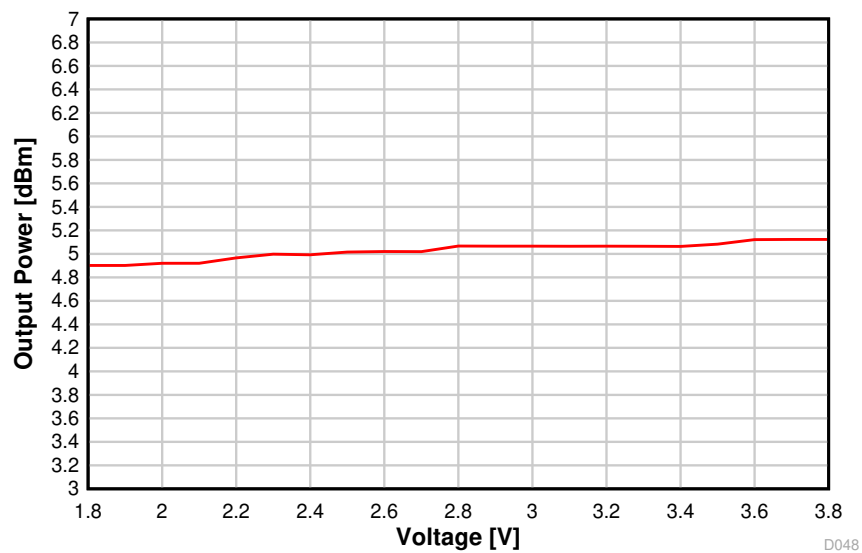
图 8-17. Output Power vs. Supply Voltage (VDD5) (BLE 1 Mbps, 2.44 GHz, +5 dBm)
