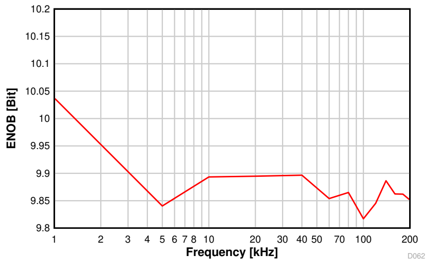
图 8-21. ENOB vs. Sampling Frequency
