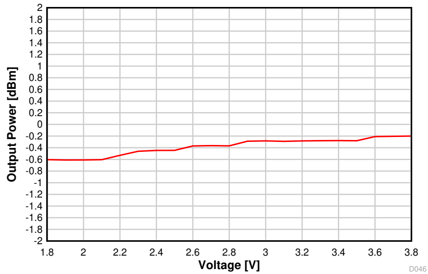
图 8-16. Output Power vs. Supply Voltage (VDD5) (BLE 1 Mbps, 2.44 GHz)
