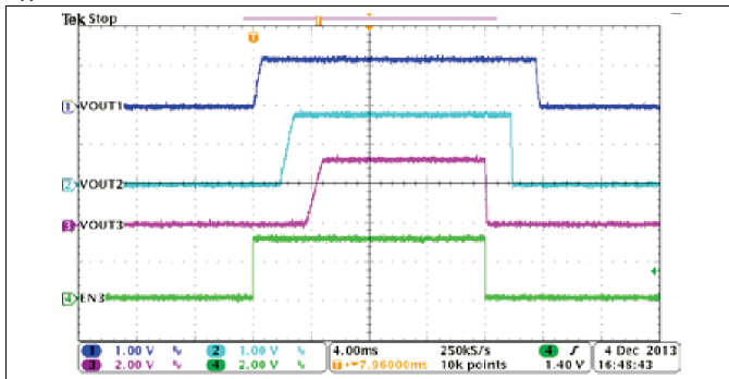
Figure 55. Automatic Power Sequencing, MODE = EN1 = EN2 = HIGH
