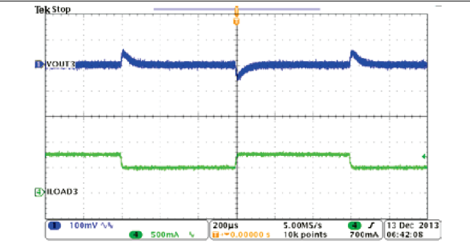
Figure 46. Buck2, Load Transient, 0.5 to 0.75 A SR = 0.25A/µs
