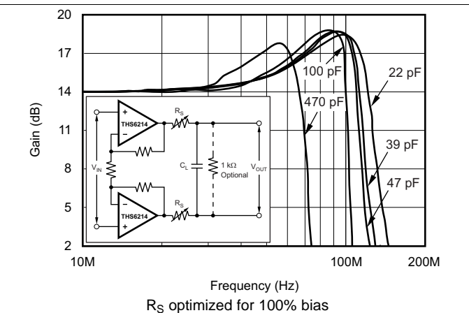
Figure 73. Frequency Response vs Capacitive Load
