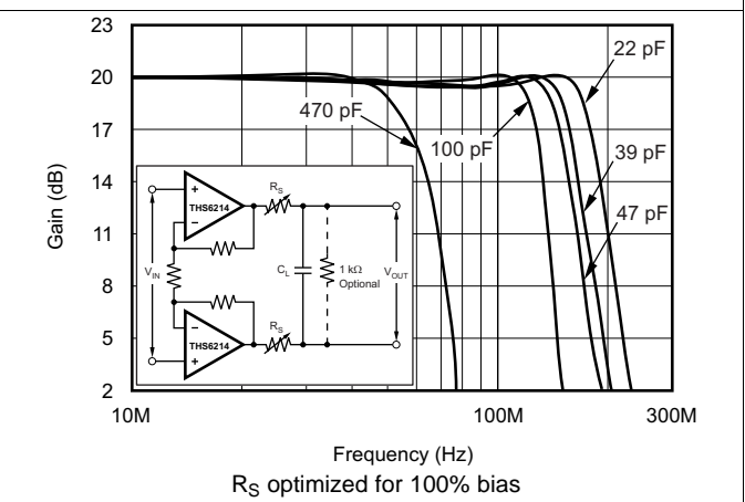
Figure 6. Frequency Response vs Capacitive Load
