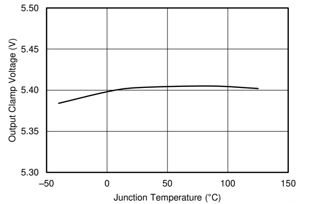
图 6-6. V_{O(VC)} vs Junction Temperature
