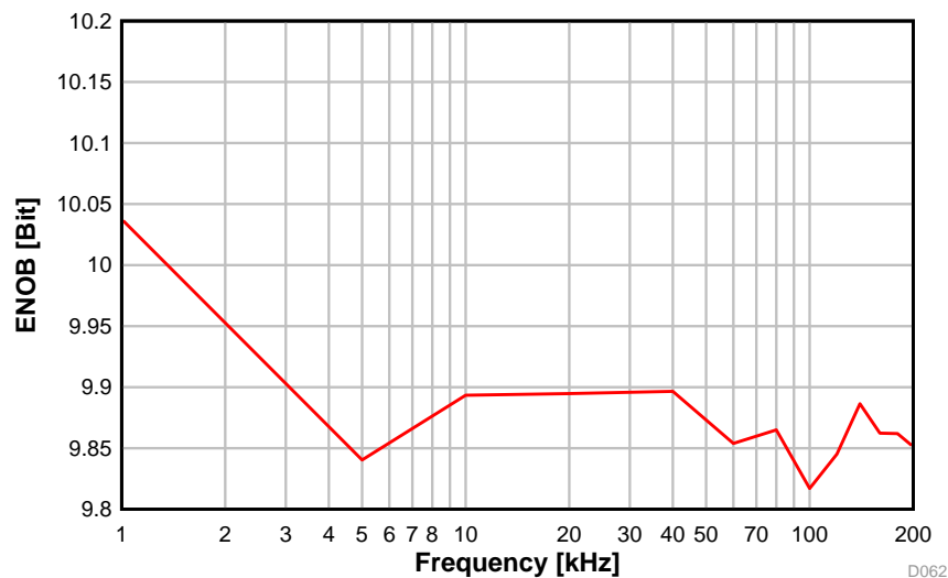
图 5-25. ENOB vs. Sampling Frequency
