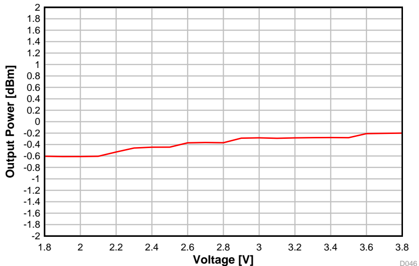
图 5-20. Output Power vs. Supply Voltage (VDDS) (BLE 1 Mbps, 2.44 GHz)
