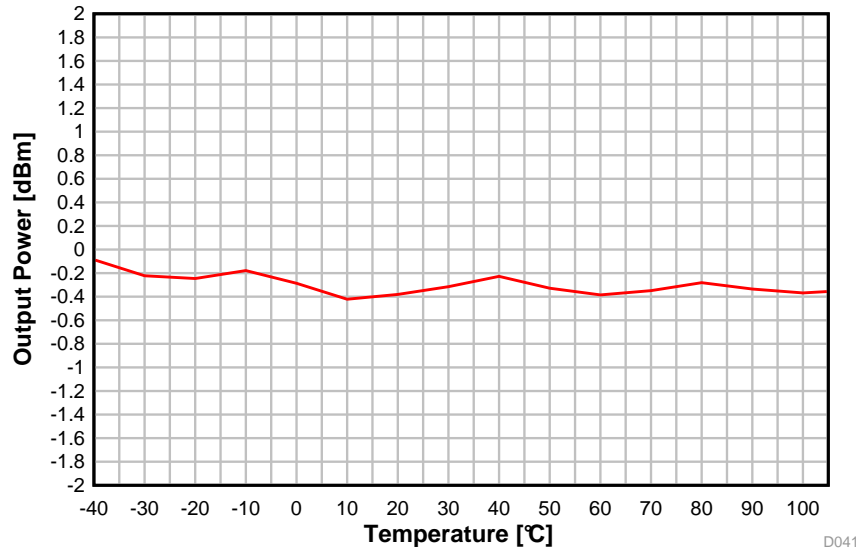
图 5-18. Output Power vs. Temperature (BLE 1 Mbps, 2.44 GHz)
