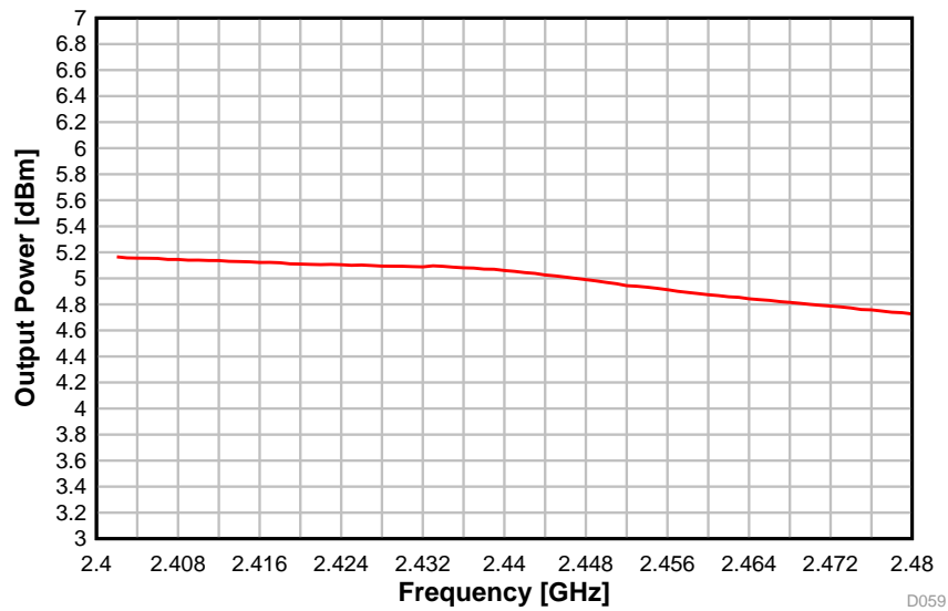
图 5-23. Output Power vs. Frequency (BLE 1 Mbps, 2.44 GHz, +5 dBm)
