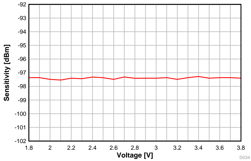
图 5-15. Sensitivity vs. Supply Voltage (VDDS) (BLE 1 Mbps, 2.44 GHz)
