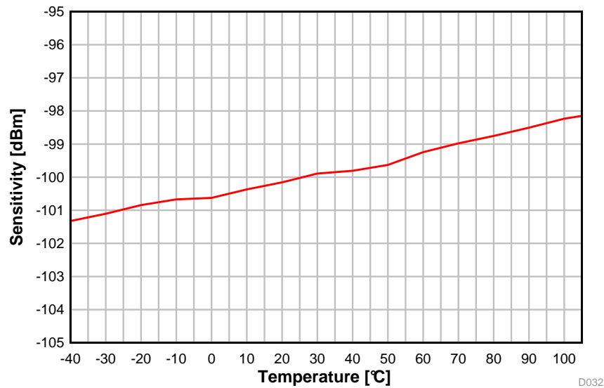
图 5-14. Sensitivity vs. Temperature (250 kbps, 2.44 GHz)
