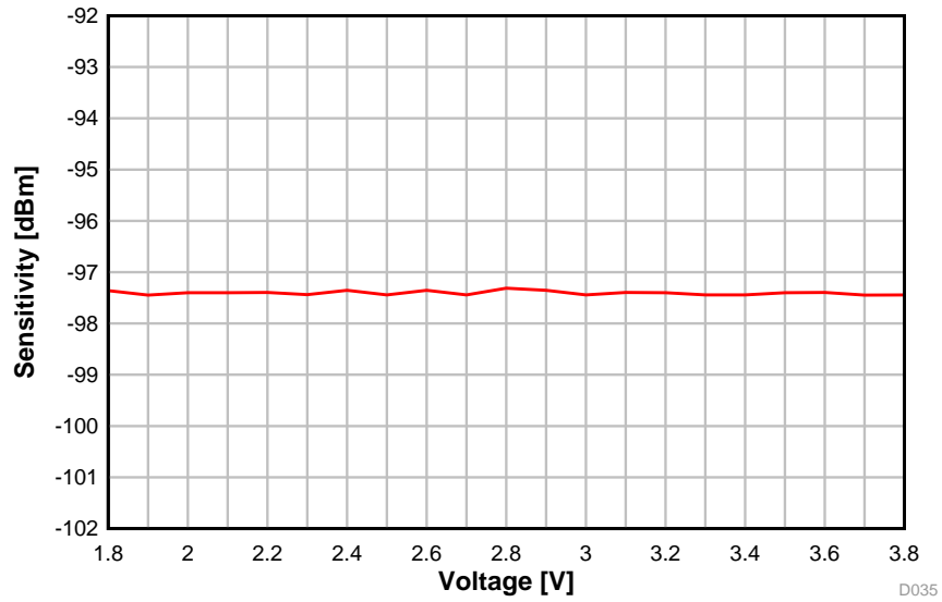
图 5-16. Sensitivity vs. Supply Voltage (VDDS) (BLE 1 Mbps, 2.44 GHz, DCDC Off)
