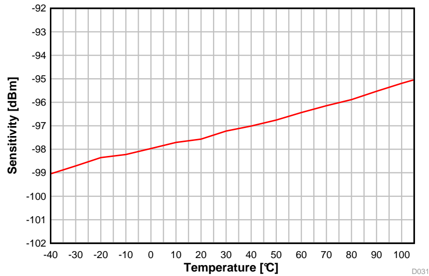
图 5-13. Sensitivity vs. Temperature (BLE 1 Mbps, 2.44 GHz)
