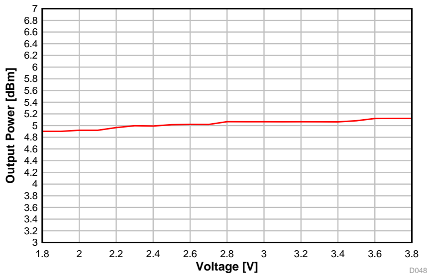
图 5-21. Output Power vs. Supply Voltage (VDDS) (BLE 1 Mbps, 2.44 GHz, +5 dBm)
