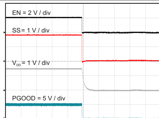
图 56. V_{DD} Shutdown Relative to Enable
