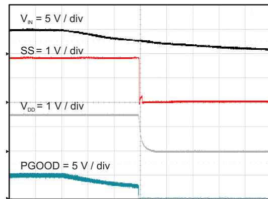
图 58. V_{DD} Shutdown Relative to V_{IN}
