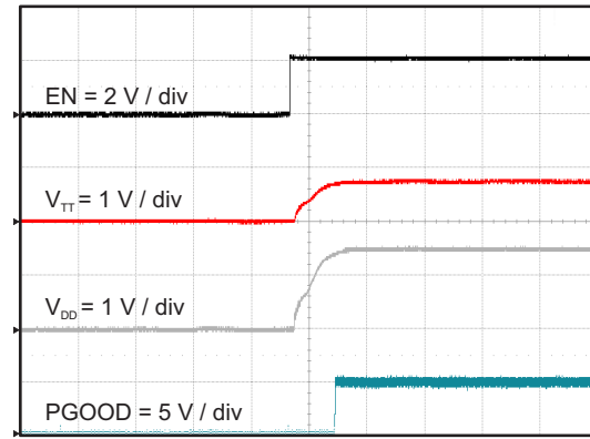
图 54. V_{TT} and V_{DD} Start-Up Relative to Enable
