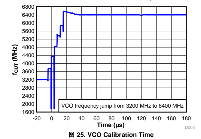
f_{VCO} = 6397 \text{ MHz} ; f_{PD} = 100 \text{ MHz} ; 3^{\text{rd}} order modulator; Fractional denominator = 1000; Loop filter bandwidth = 115 kHz
