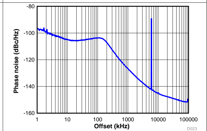
f_{VCO} = 6397 \text{ MHz} ; f_{PD} = 100 \text{ MHz} ; 3^{\text{rd}} order modulator; Fractional denominator = 2^{32} - 1 ; Loop filter bandwidth = 115 kHz
