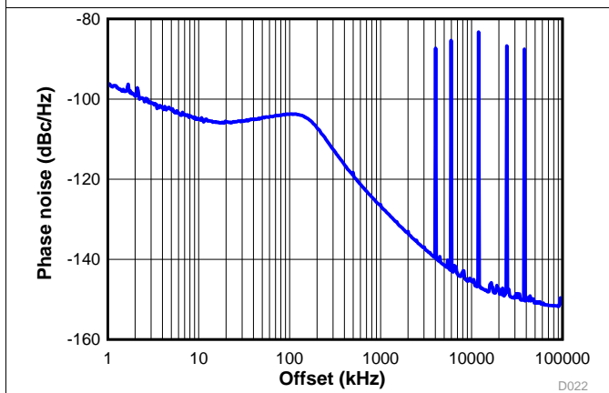
f_{VCO} = 6397 \text{ MHz} ; f_{PD} = 100 \text{ MHz} ; 3^{\text{rd}} order modulator; Fractional denominator = 1000; Loop filter bandwidth = 115 kHz
