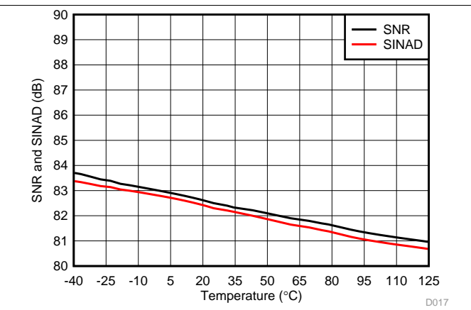
Figure 18. Signal-to-Noise Ratio and Signal-to-Noise + Distortion vs Temperature
