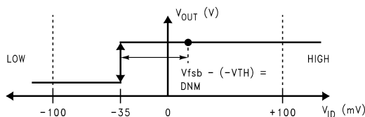
Figure 21. VTC of the DS90LV028A
