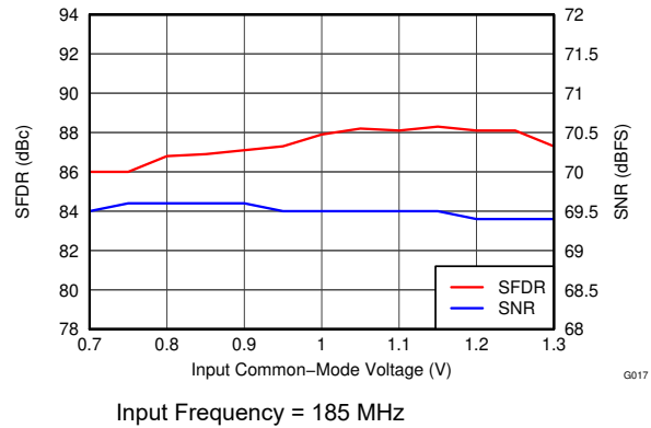
图 6-19. Performance vs Input Common-Mode Voltage
