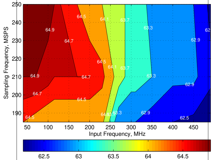
图 6-37. Signal-to-Noise Ratio (6-dB Gain)
