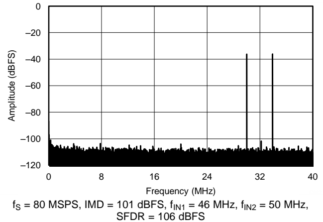
Figure 78. FFT for Two-Tone Input Signal ( -36\text{ dBFS} at 46 MHz and 50 MHz)
