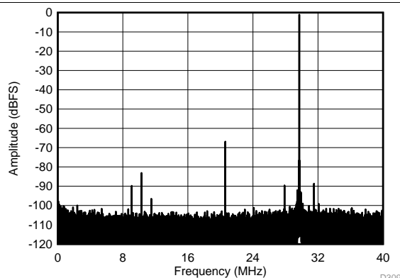
SFDR = 66 dBc, SNR = 68.4 dBFS, SINAD = 64.6 dBFS, THD = 66 dBc, HD2 = 66 dBc, HD3 = 89 dBc
