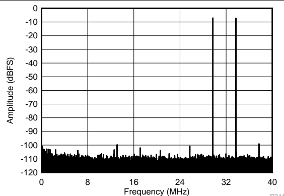
f_{IN1} = 46 \text{ MHz} , f_{IN2} = 50 \text{ MHz} , IMD3 = 99 dBFS, each tone at -7 dBFS
