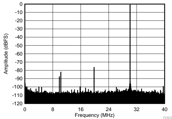
SFDR = 75 dBc, SNR = 70.5 dBFS, SINAD = 69.6 dBFS, THD = 74 dBc, HD2 = 75 dBc, HD3 = 81 dBc
