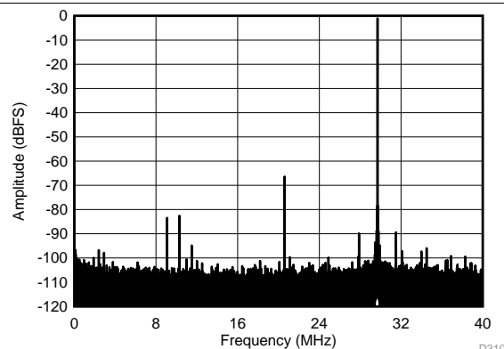
SFDR = 65 dBc, SNR = 68.7 dBFS, SINAD = 64.4 dBFS, THD = 65 dBc, HD2 = 65 dBc, HD3 = 82 dBc
