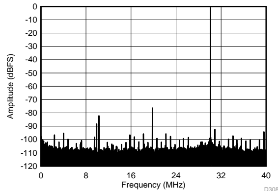
SFDR = 75 dBc, SNR = 71 dBFS, SINAD = 69.7 dBFS, THD = 74 dBc, HD2 = 75 dBc, HD3 = 81 dBc
