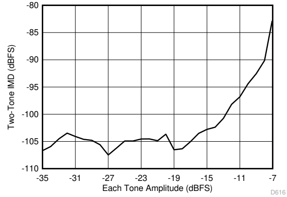
图 6-46. Intermodulation Distortion vs Input Amplitude (185 MHz and 190 MHz)
