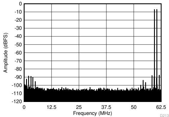
f_{IN1} = 185\text{ MHz} , f_{IN2} = 190\text{ MHz} , \text{IMD3} = 87.5\text{ dBFS} , each tone at -7 dBFS
