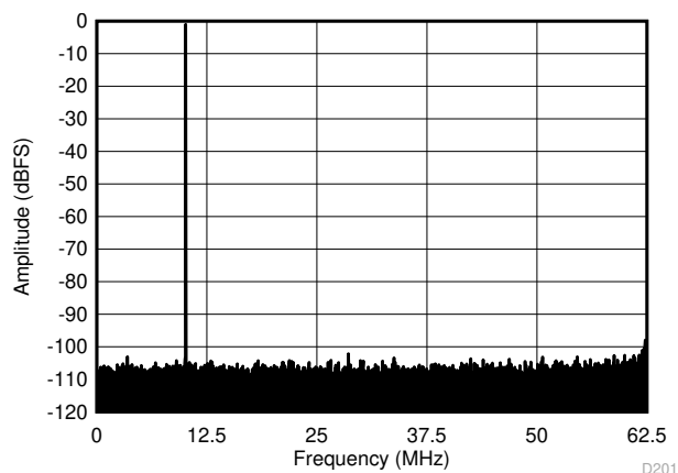
图 9-4. Performance FFT at 10 MHz (Low Input Frequency)
