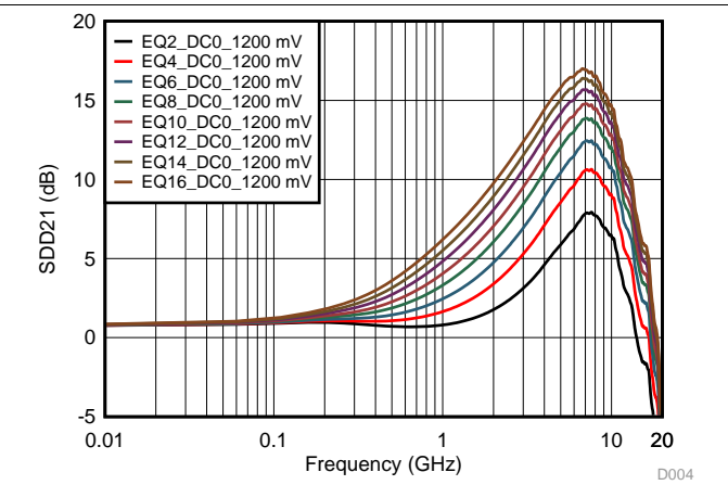
图 4. 1200 mV DC0 Even EQ Settings Curves
