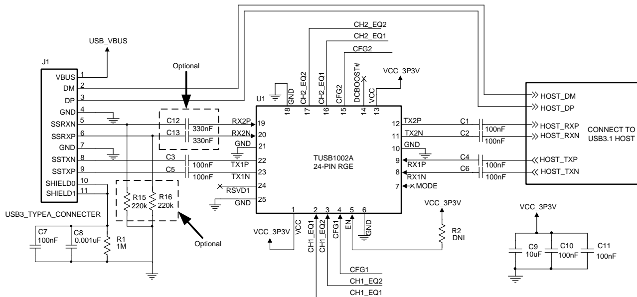
图 18. Host Implementation Schematic
