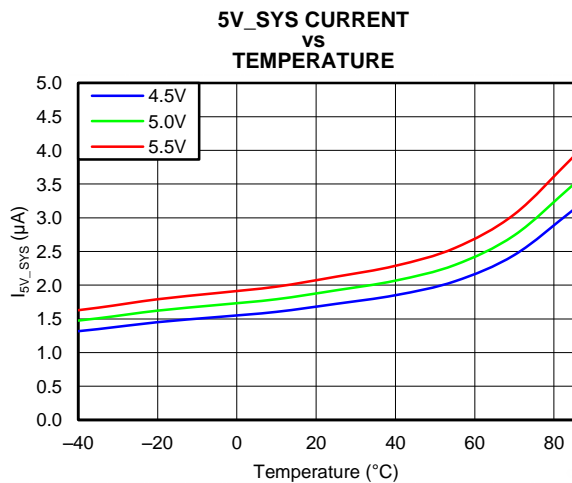
Figure 13. I_{5V\_SYS} Data
