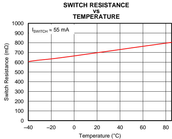
Figure 12. Rds Data
