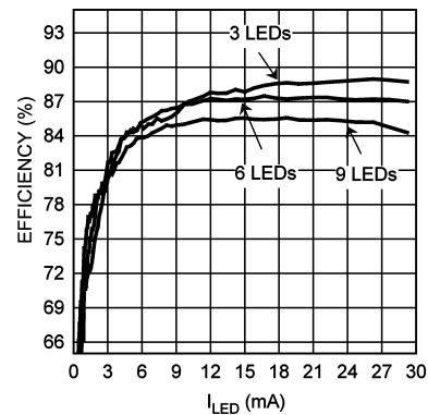
Figure 53. Efficiency vs I_{LED}
